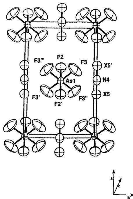
Figure 1. A unit cell plot of \text{N}_2\text{F}^+\text{AsF}_6^- viewed down the c axis. In addition to the mirror plane, 2-fold rotational axes pass through As1 (bisecting the F3-As1-F3' angle) and N4 (perpendicular to the X5-N4-X5' axis). The \text{N}_2\text{F}^+ cation is required by symmetry to be disordered, with the terminal X5, X5' positions being occupied equally by N and F atoms. This packing disorder causes the \text{NX}_2 cation to be linear and symmetric, and the central nitrogen atoms to be elongated along the molecular axis.
