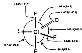
Figure 3. Geometry of \text{ClF}_3\text{O} (bond lengths in angstroms, angles in degrees) as calculated by the LDF method. The experimentally observed 32 values are given in parentheses.
