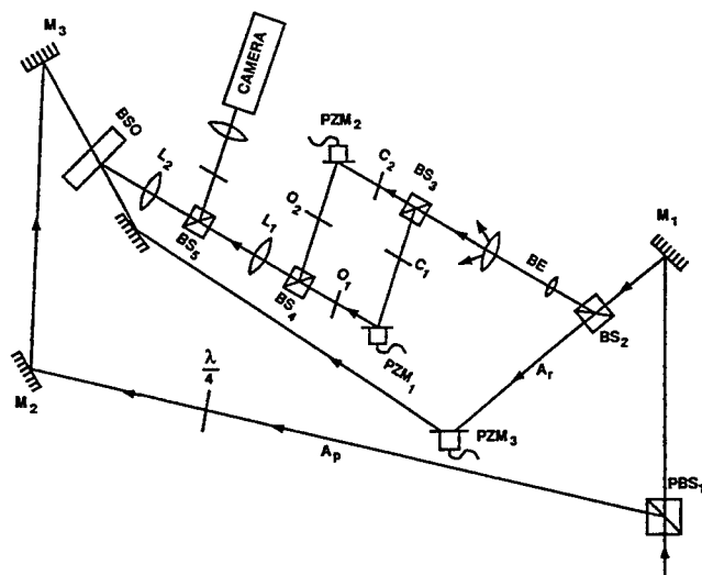
Fig. 2. Experimental setup for optical demultiplexing (see text). The modulation of the beams is accomplished through piezoelectric transducers PZM_1 – PZM_3 . The baseband signal is generated by choppers C_1 and C_2 . O's, transmissive objects; M's, mirrors; L's, lenses; BS's, beam splitters; BE, beam expander; PBS 1 , polarizing beam splitter; \lambda/4 , quarter-wave plate.
