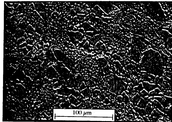
MICROSTRUCTURE AFTER PRESSING
