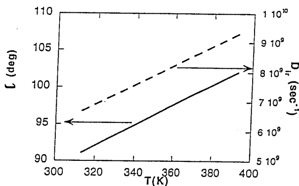
Figure 5. l and D_{lr} as a function of temperature; values from the Hall-Helfand model.
