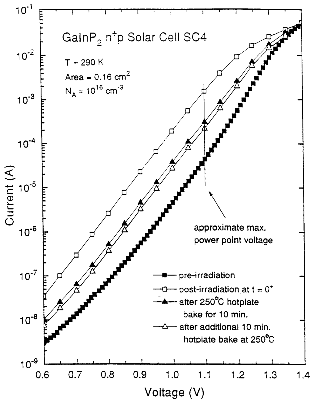
Figure 67. Forward-bias dark I-V curves for a \text{GaInP}_2 n + p solar cell before and after 1 MeV electron irradiation and thermal annealing at 250^\circ\text{C} .
