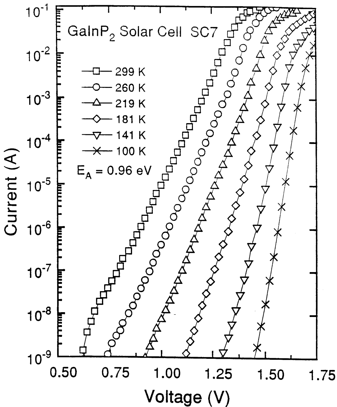
Figure 27. Forward-bias dark I-V curves as a function of temperature for a "well-behaved" GalnP 2 solar cell.
