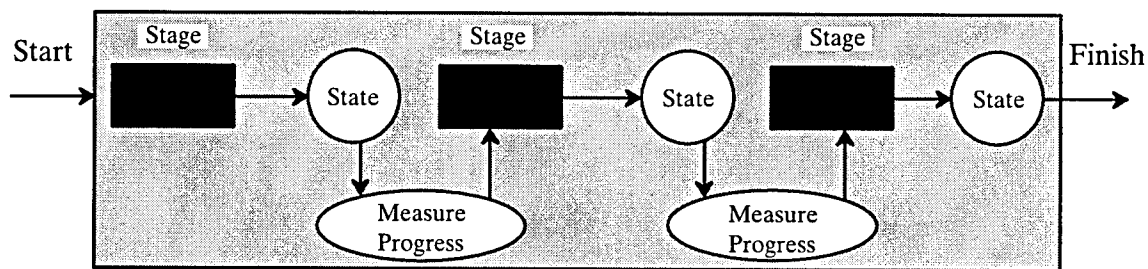
Figure 2. Life-Cycle Model
