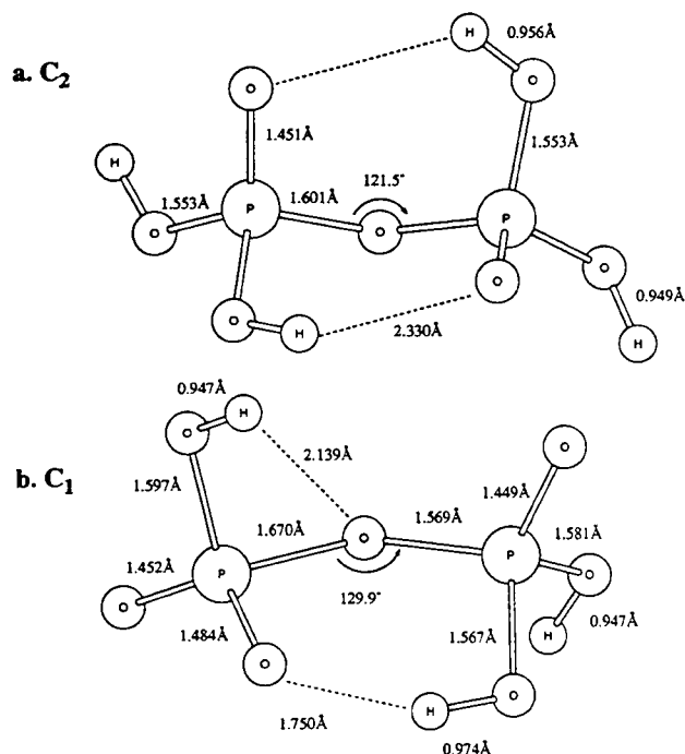
Figure 1. Equilibrium geometries of (a) pyrophosphoric acid H_4P_2O_7 and (b) pyrophosphorate monoanion H_3P_2O_7^- at the DZP SCF level.
