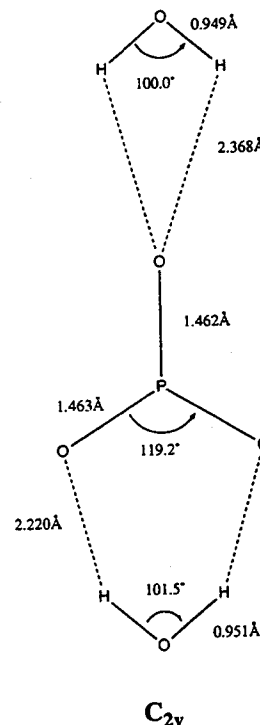
Figure 10. A transition state for PO 3 - ·(H 2 O) 2 optimized at the DZP SCF level of theory.
