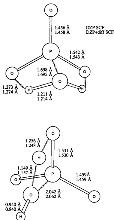
Figure 1. Two C_{2v} symmetry stationary points (each with two imaginary vibrational frequencies) related to the isomerization of \text{PO}_3^{2-}\cdot\text{H}_2\text{O} to \text{H}_2\text{PO}_4^{2-} .
