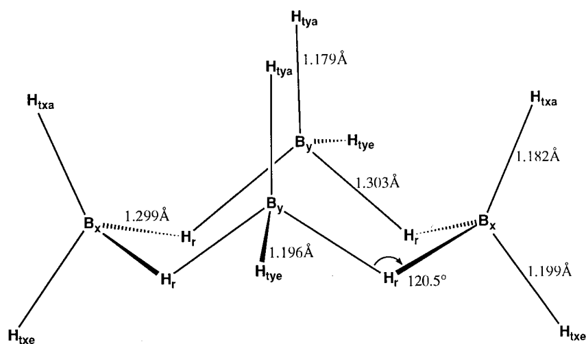
Fig. 2. C 2v deformed ring (or "butterfly") structure for tetraborane(12) B 4 H 12 . This structure is energetically lowest lying and a local minimum on the SCF potential energy surface. The B-H-B bridge bonds are pronouncedly bent. The indicated geometrical parameters were obtained at the DZP CCSD level of theory.
