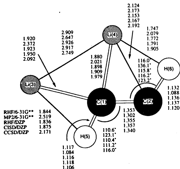
Figure 8. Summary of theoretical geometries for structure 6, the ^1A transition state of the trans -1,2-dilithioethene molecule that interconverts structures 1 and 7, and an electrostatic interpretation with a qualitative representation of the canonical HOMO superimposed. Bond distances are in angstroms, and bond angles are in degrees.
