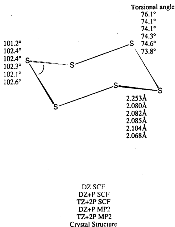
Figure 1. Predicted D_{3d} equilibrium geometries for S_6 .
