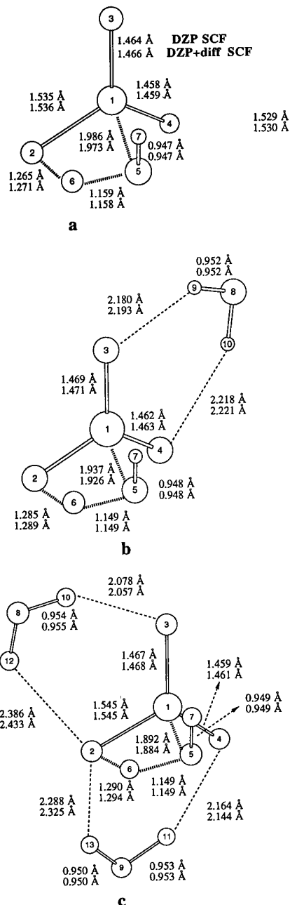
Figure 2. The four-center transition states from \text{PO}_3^{2-}(\text{H}_2\text{O})_n to \text{H}_2\text{PO}_4^{2-}(\text{H}_2\text{O})_{n-1} : (a) \text{PO}_3^{2-}\cdot\text{H}_2\text{O} to \text{H}_2\text{PO}_4^{2-} ; (b) \text{PO}_3^{2-}(\text{H}_2\text{O})_2 to \text{H}_2\text{PO}_4^{2-}\cdot\text{H}_2\text{O} ; (c) \text{PO}_3^{2-}(\text{H}_2\text{O})_3 to \text{H}_2\text{PO}_4^{2-}(\text{H}_2\text{O})_2 .
