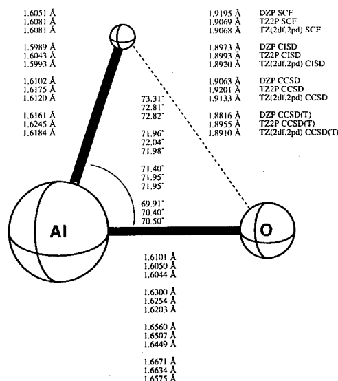
FIG. 3. Predicted structure for C_s -symmetry transition state for the \tilde{X} AlOH \leftrightarrow \tilde{X} HAIO isomerization reaction.
