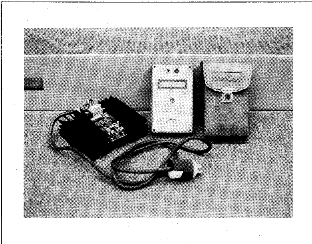
Figure 6. Pulse generator and waveform analyzer model WFA-1.
