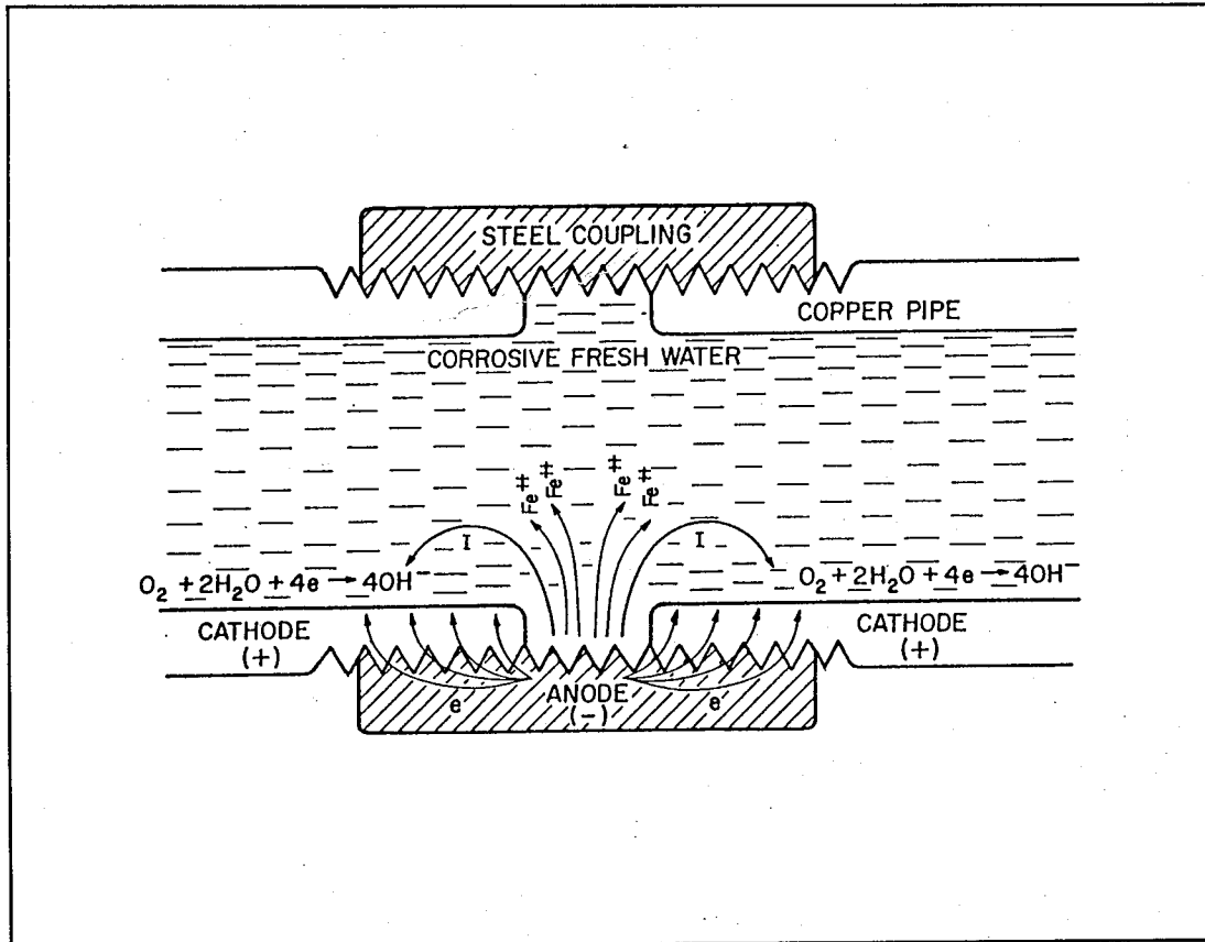
Figure 1. A typical corrosion cell.
