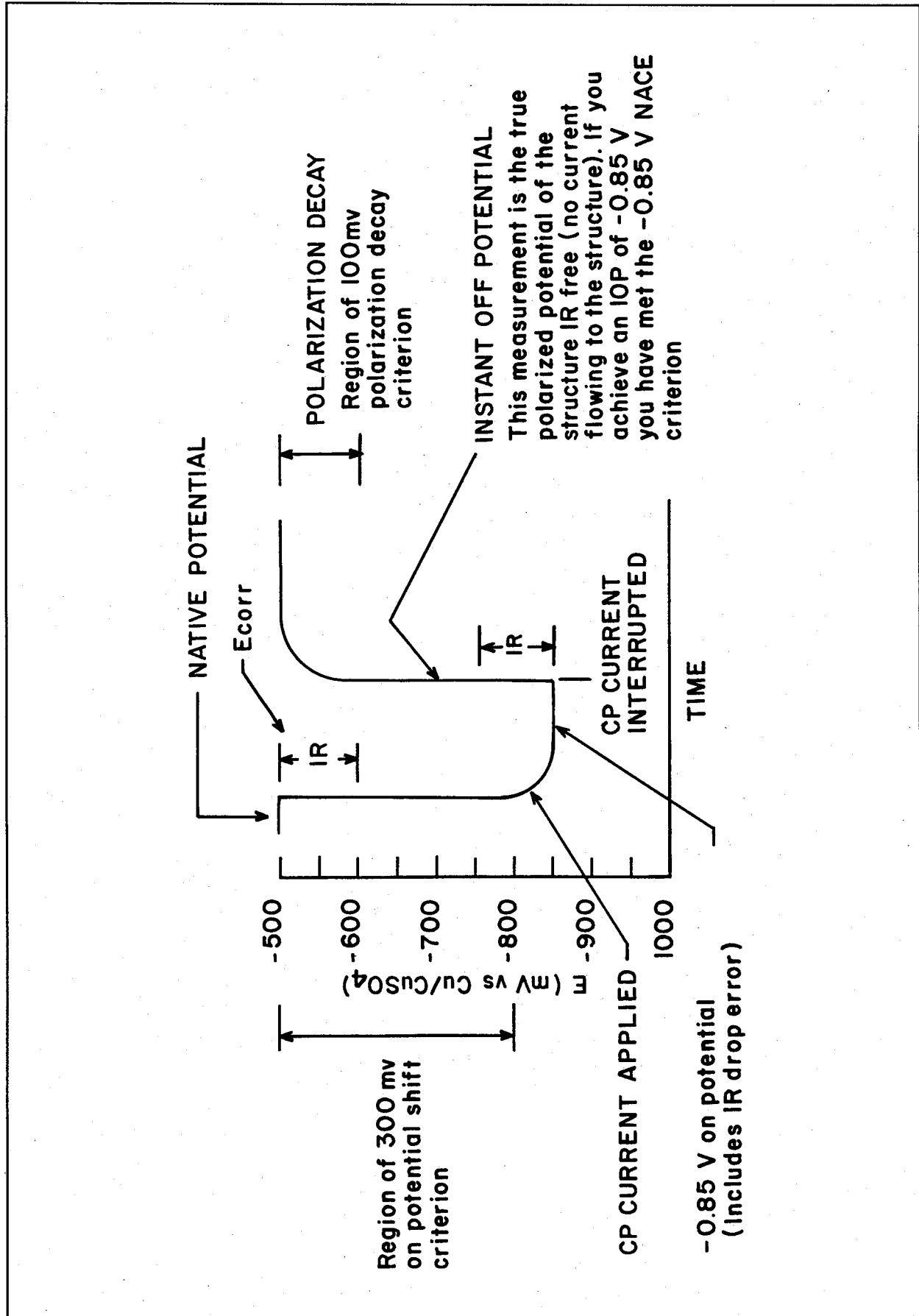
Figure 3. Potential and potential shift criteria for cathodic protection of steel.
