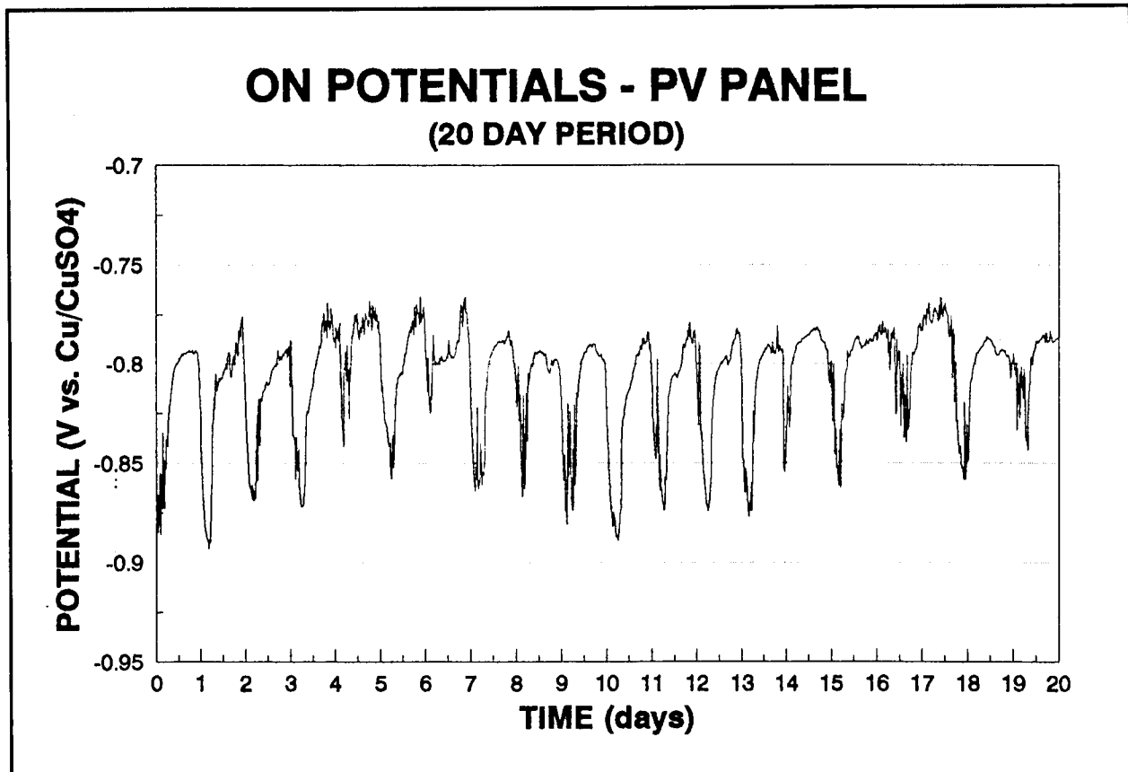
Figure 23. On-potential vs. time for photovoltaic panel for 20-day period.
