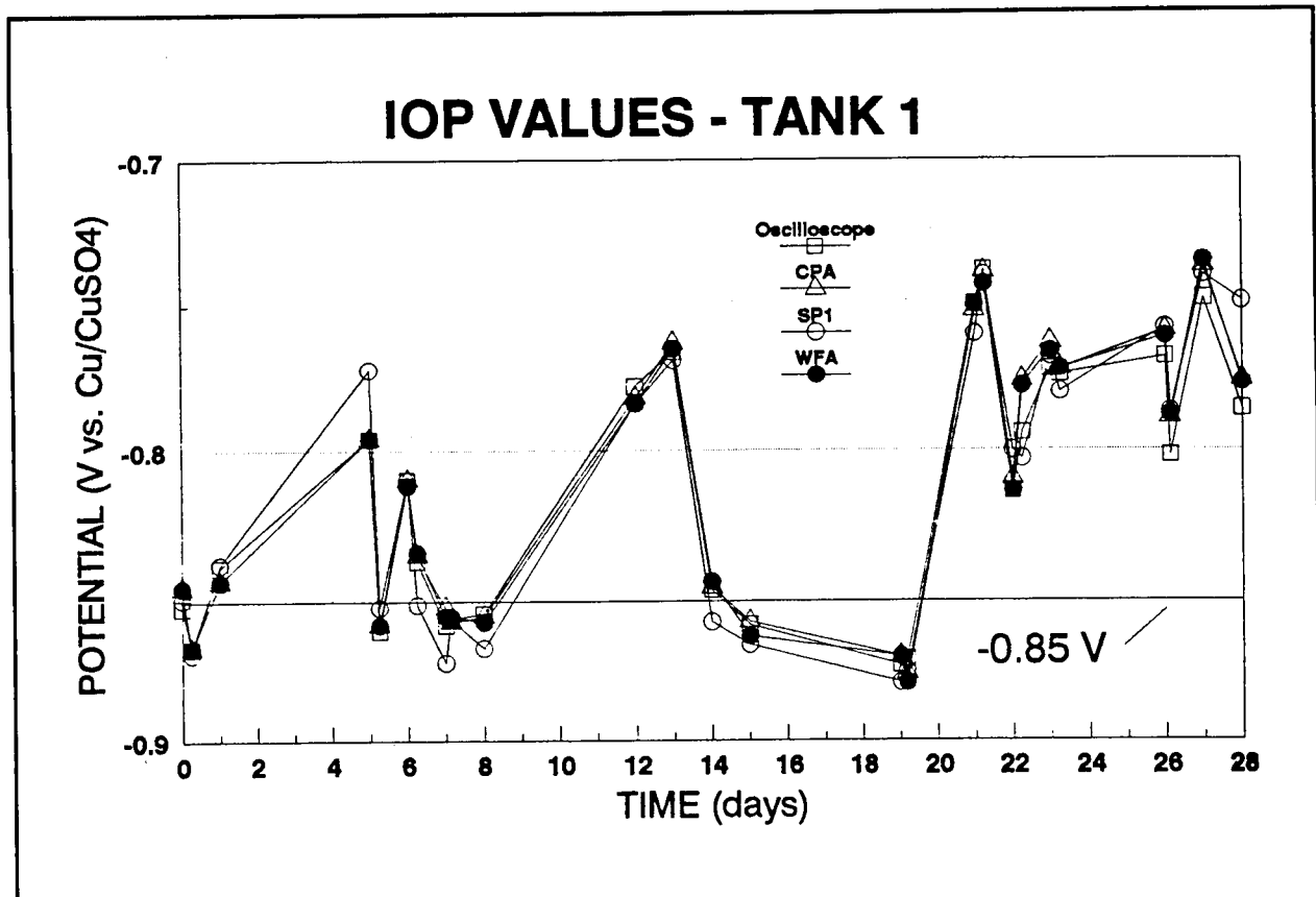
Figure 20. Off-potentials vs. time for Tank 1.
