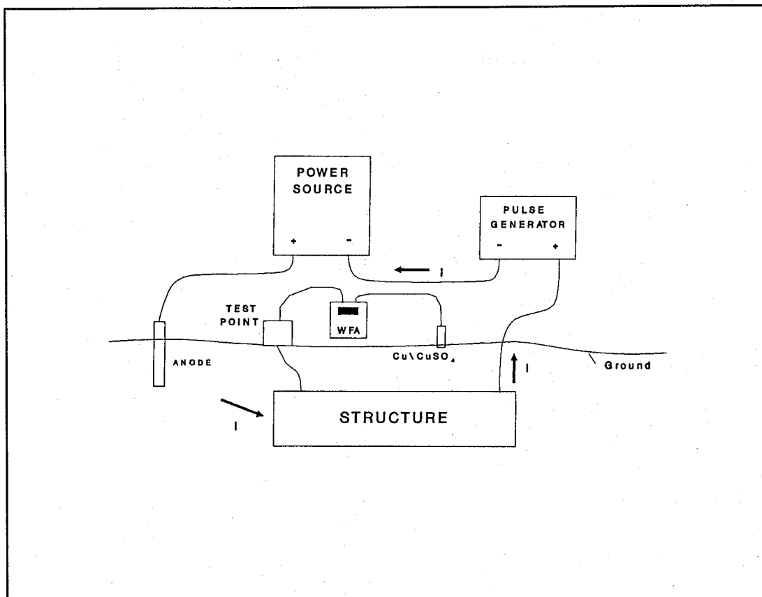
Figure 7. Waveform analyzer/pulse generator measurement system.
