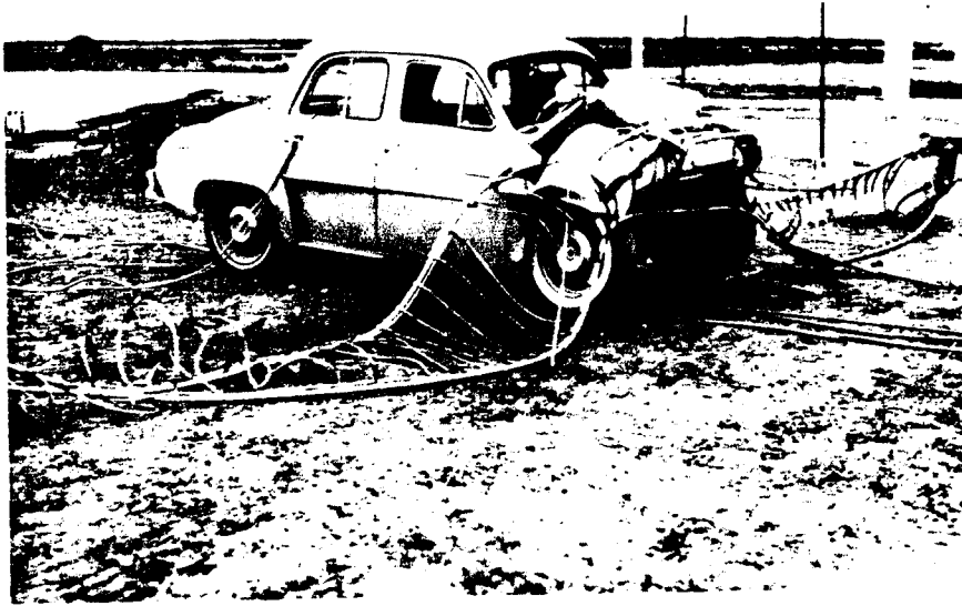
Figure 5, Vehicle and Dragnet after Test 505-4A.
