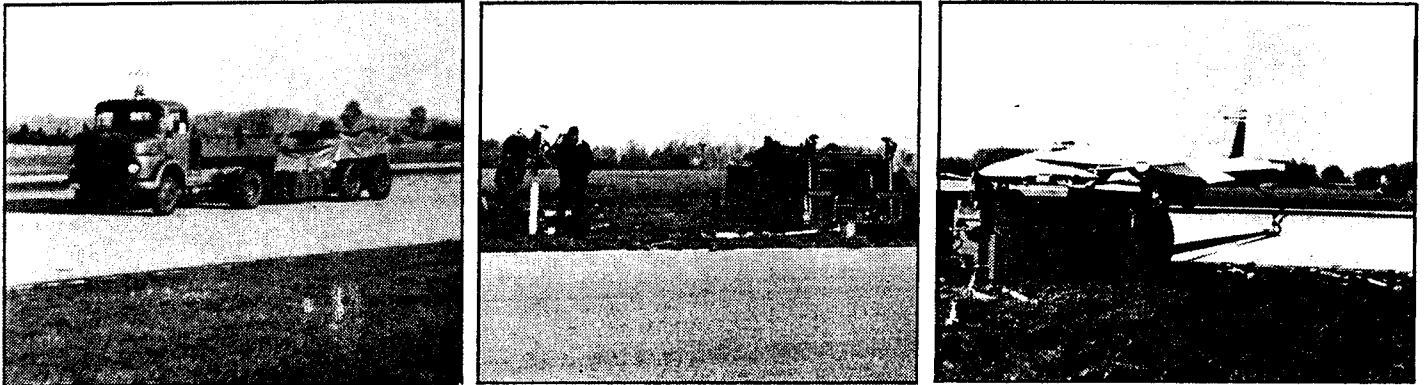
Figure 9. Mobile Arresting Gear (F-18 Aircraft)
