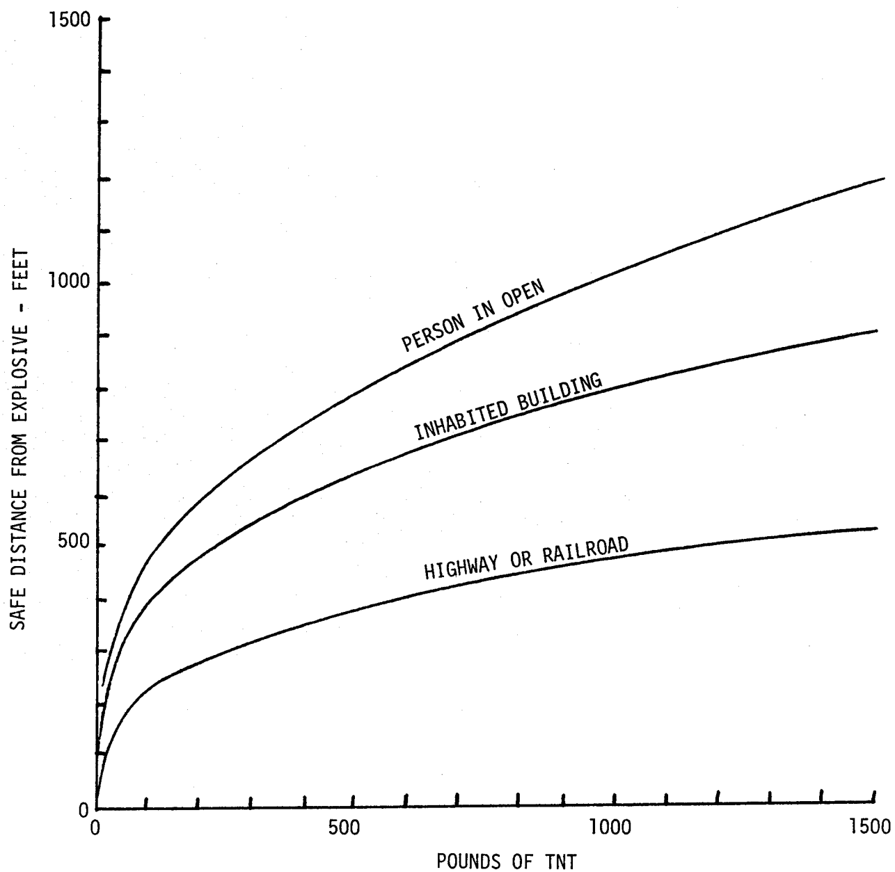
FIGURE 15. SAFE DISTANCE FROM EXPLOSION - NO BARRICADE (from Ref. 26)
