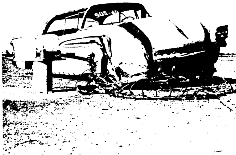
Figure 15, Vehicle and Right Metal Bender After Test 505-4D.
