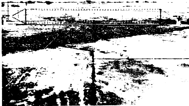
Figure 7 , Arresting System Before Test 505-4B. (Looking Along Path of Vehicle)
