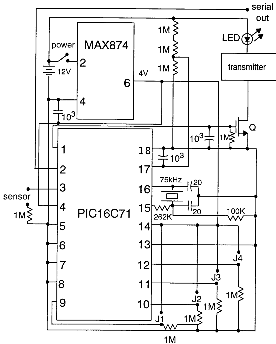
Figure 4. Monitor Electronics
