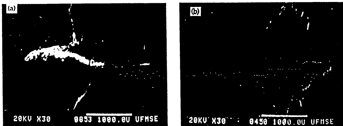
Fig. 8—An edge view of tensile tested specimens. (a) Debonding at the interface in a specimen with \text{Al}_2\text{O}_3 coated Nb. (b) Multiple matrix fracture near the interface in a specimen with uncoated Nb.
