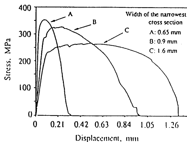
Fig. 10 Stress-displacement curves for different sizes of constrained Nb laminae. The thickness of the Nb laminae is 0.25, 0.5 and 1.0 mm for curves A, B and C, respectively
