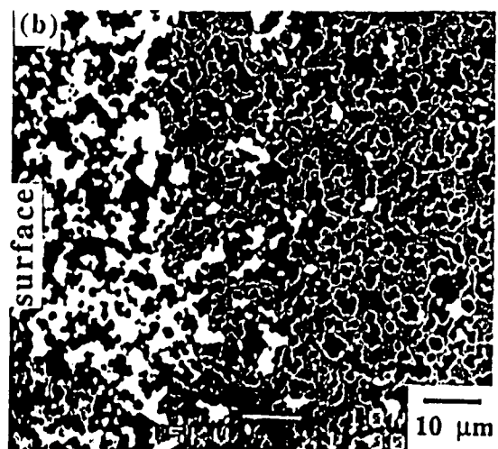
Fig. 2.(a) Equilibrium dissociation pressures of Si over MoSi 2 , as adapted from [12]. (b) BEI of the surface of a MA40 sample hot pressed at 1700°C, showing silicon depletion. Light phase is the Nowotny phase, grey phase is MoSi 2 and dark phase is SiC.
