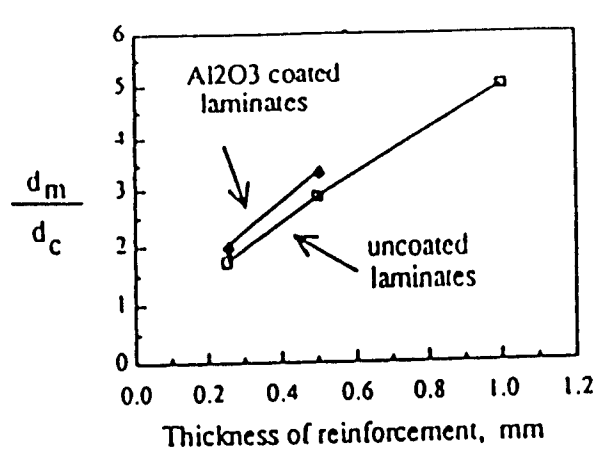
Fig. 5 A plot of ratio of the measured to characteristic decohesion length as a function of reinforcement size.
