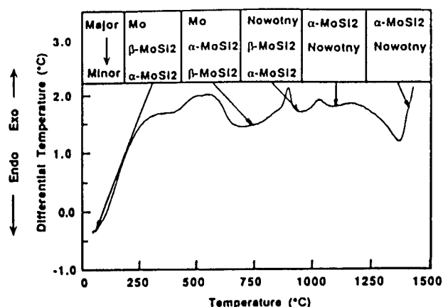
FIG. 8. DTA of ternary MoSi 2 under flowing argon at a heating rate of 10 °C/min, along with the corresponding phases identified by XRD. ("Nowotny" refers to the Nowotny phase, C 41 Mo 45 Si 3 .)
