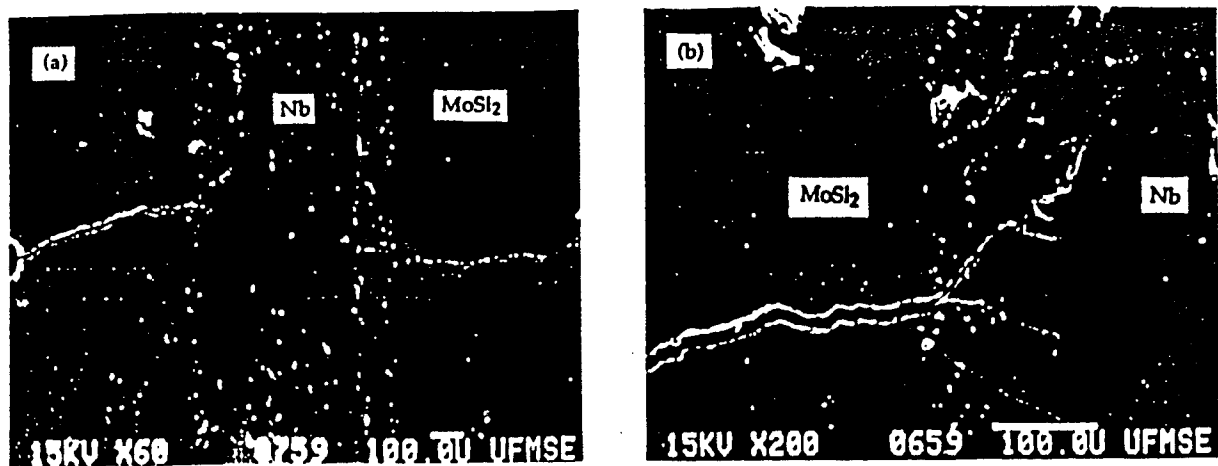
Fig. 6—An edge view of an unloaded tensile test specimen. (a) A general view of the cracks and (b) a close-up of the crack tips showing dislocation slip of the Nb at the crack tips.
