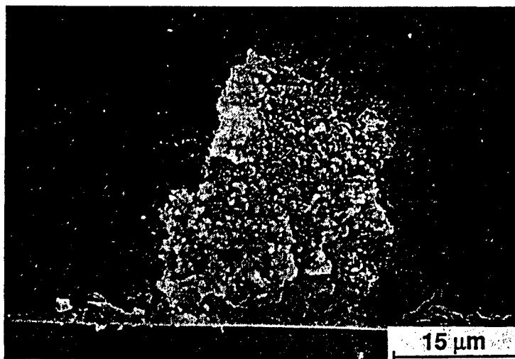
FIG. 6. SEM micrograph of a fracture surface of a \text{SiO}_2/\text{Si}_3\text{N}_4 sample (sintered at 1300^\circ\text{C} , 2 h) showing a large processing defect (powder agglomerate).
