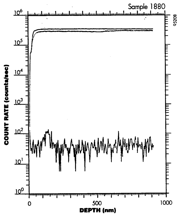
Figure 5 (Cont.) SIMS of samples 1878, 1879, and 1880, demonstrating variation of erbium doping with process variables (Table 2).
