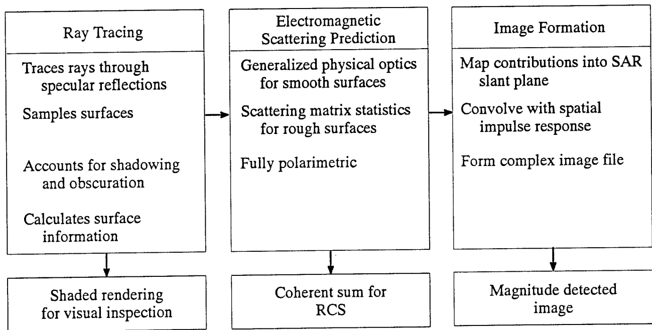
Figure 6. SRIM Processing
