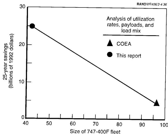
Figure 4.36—The 25-Year Savings Attributable to Buying a 747-400F Fleet Instead of 120 C-17s Is Sensitive to Analysis of Utilization Rates, Payloads, and Load Mix
