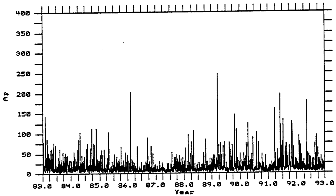
Figure 3 Magnetic Activity Daily Averaged Ap
