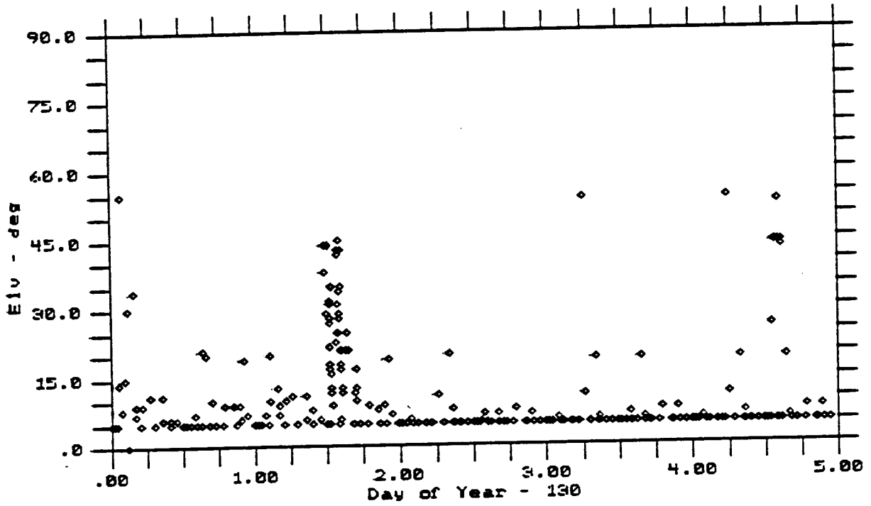
Figure 14 Loss of Locks vs Elevation Angle at South Pole for May 1992 Magnetic Storm
