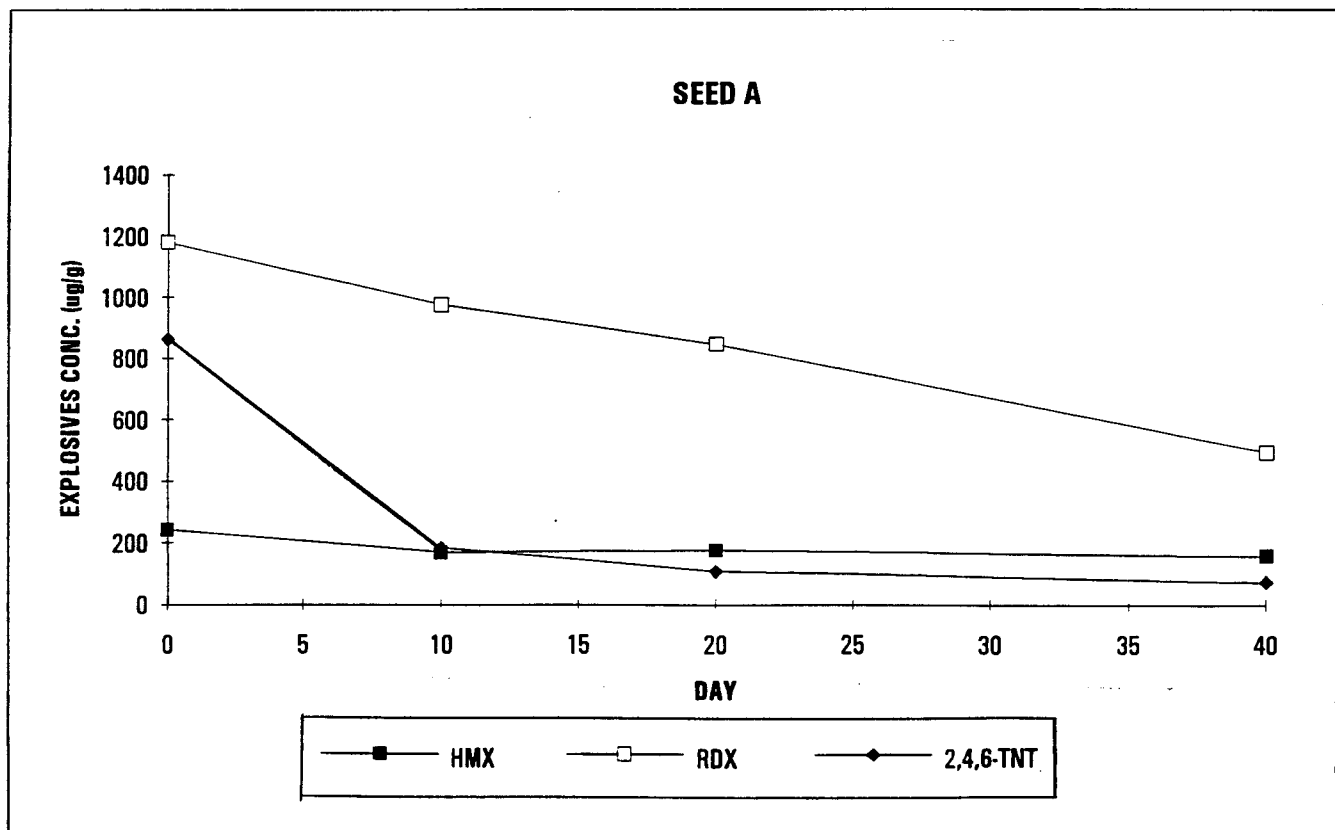
FIGURE 5-9 EXPLOSIVES CONCENTRATIONS VS. TIME FOR SEEDING STUDY A
