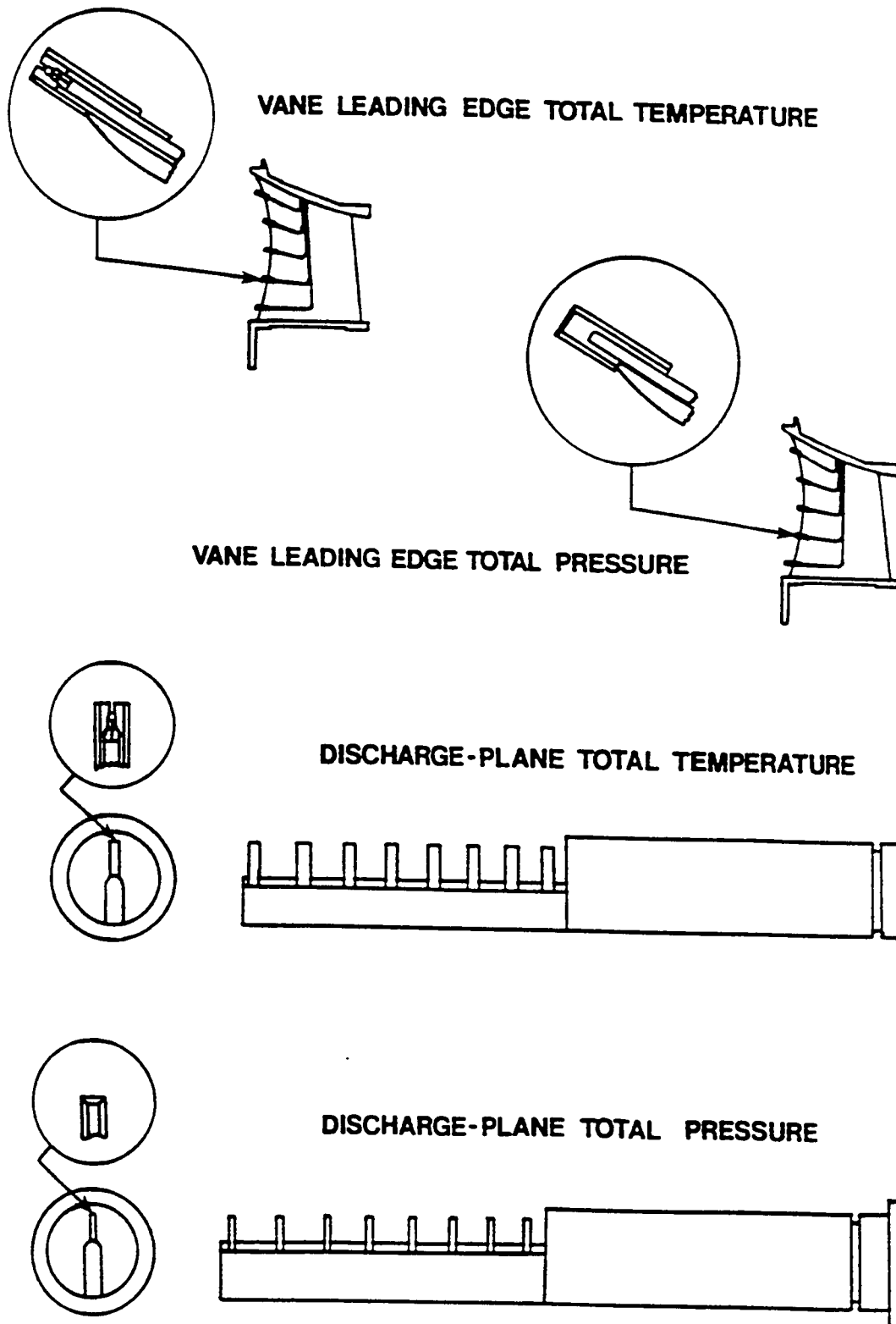
Figure 3.10 Vane Leading Edge and Discharge Plane Rake Instrumentation [29]
