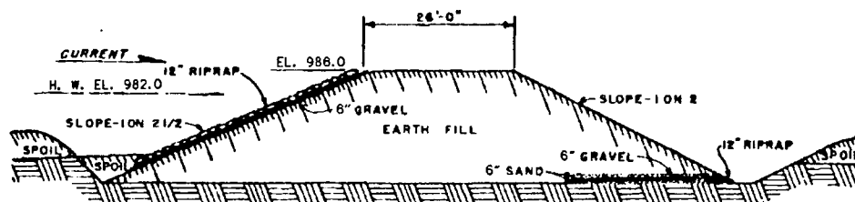
EARTH DIKE SECTION WHITE ROCK DAM 10 0 10 20 30 SCALE IN FEET
