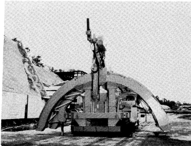
Figure B5. Concrete Spraying Robot.
