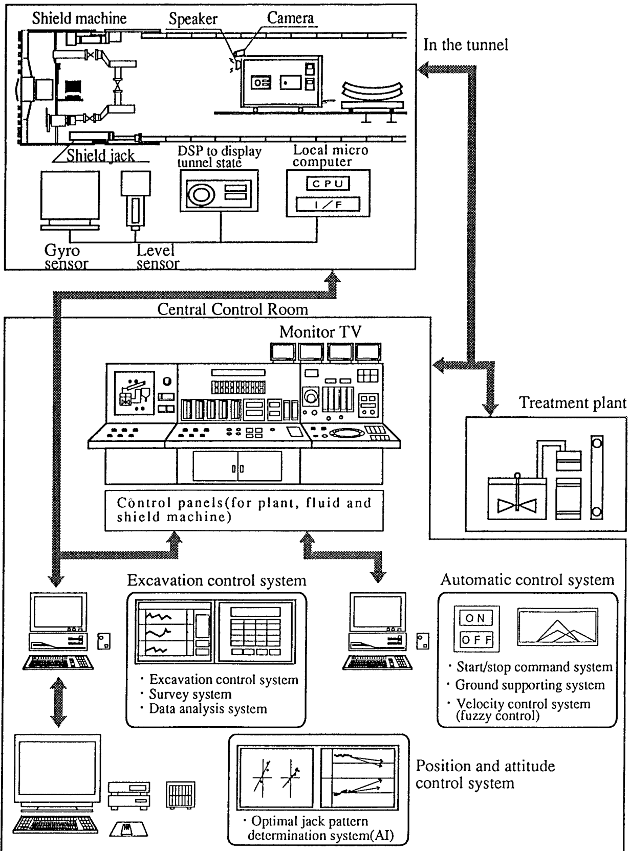
Figure A10. Automated Shield Tunneling.
