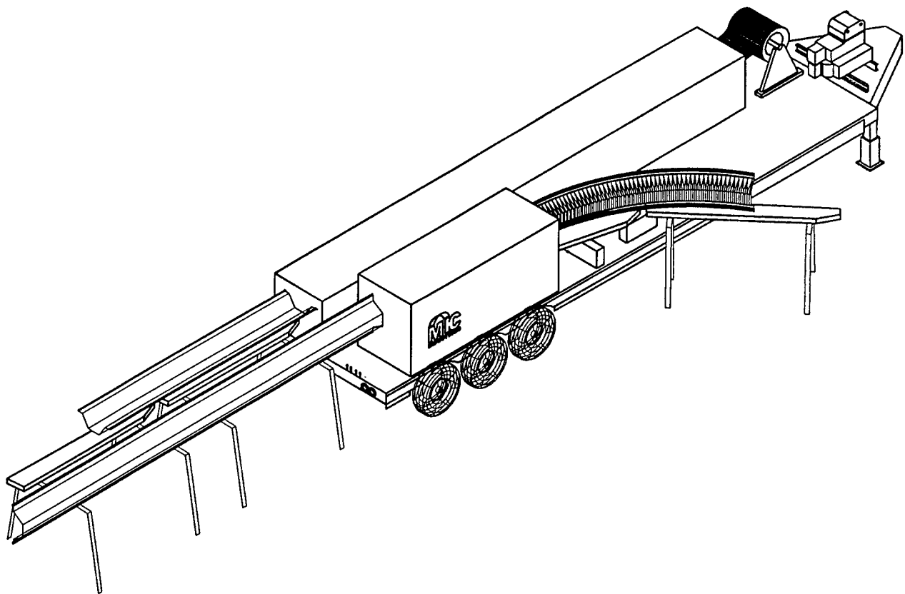
Figure E2. Automatic Building Machine (ABM)
