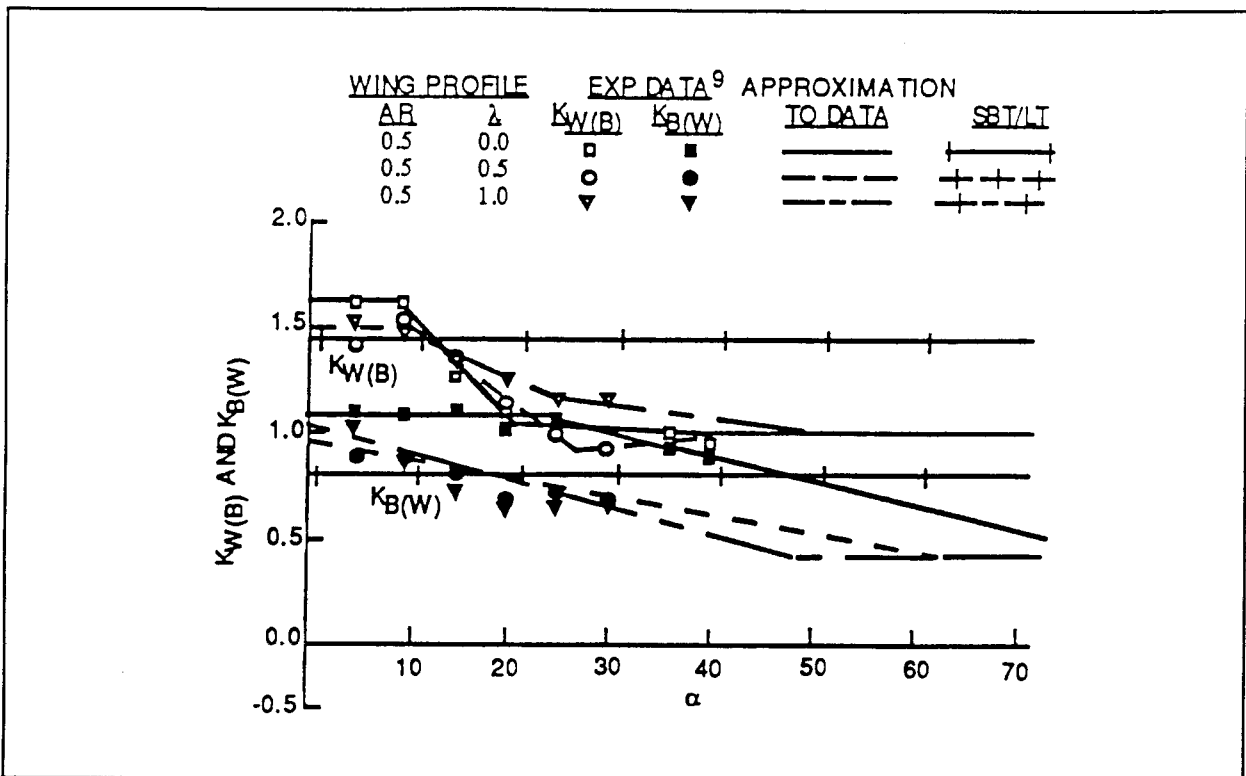
FIGURE 14. WING-BODY AND BODY-WING INTERFERENCE FACTORS AS A FUNCTION OF AOA ( M_\infty = 1.2 )
