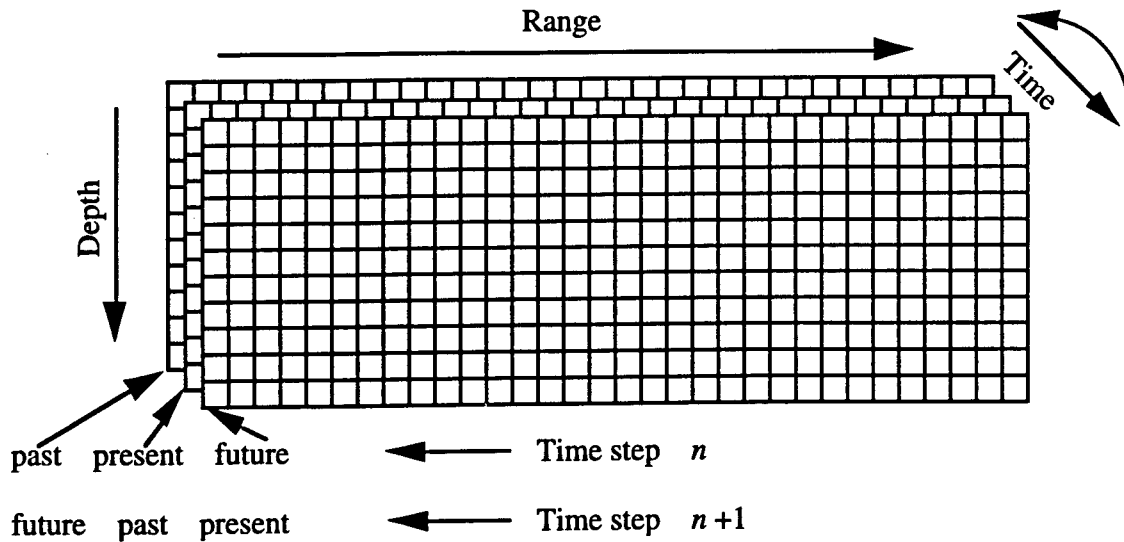
Fig. 2 — Organization of field array and time-step pointers. By rearranging the past, present, and future pointers, old results are overwritten and massive memory transfers are avoided.
