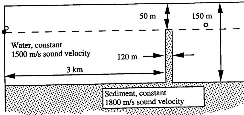
Fig. 8 — Reverberation and Scattering Workshop Test Case 2a environment. Source depth is 50 m (filled circle); receivers are located 45 m deep at 5- and 3500-m range (hollow circles). The thickness of the obstacle at 3000-m range is 2 wavelengths of the 30-Hz center frequency.
