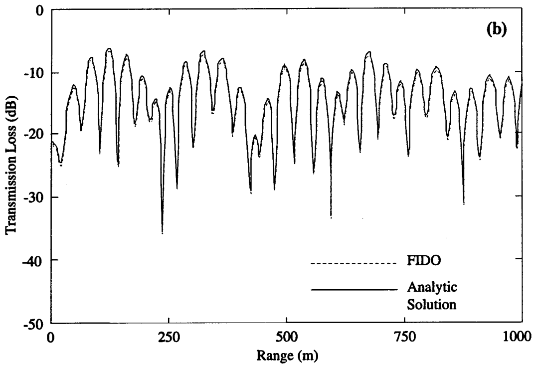
Fig. 7 — ASA ideal wedge benchmark problem solution for FIDO. First 1000 m of part (a) have been expanded and overlaid with analytic solution [8] in (b).
