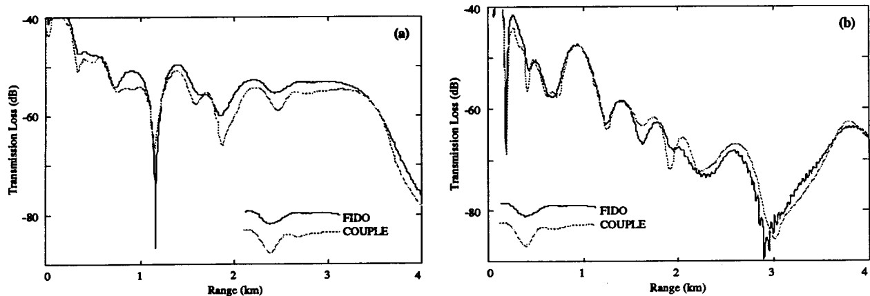
Fig. 4 — ASA penetrable loss wedge benchmark problem solutions for FIDO and COUPLE. Receiver depths are (a) 30 m and (b) 150 m.
