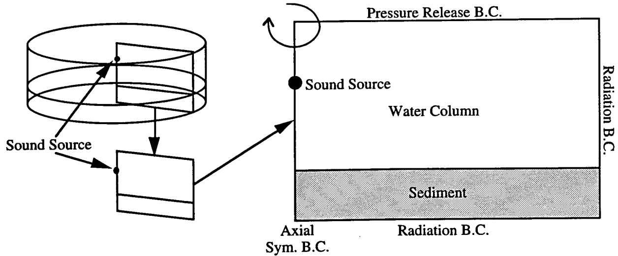
Fig. 1 — Geometry and boundaries used by FIDO and the relationship between three-dimensional axially symmetric problem and two-dimensional solution grid.
