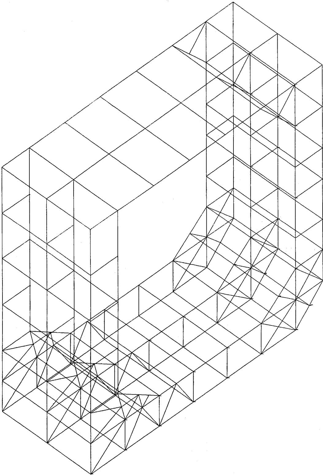
Figure A-5 Course mesh FEA model of double hull tanker
