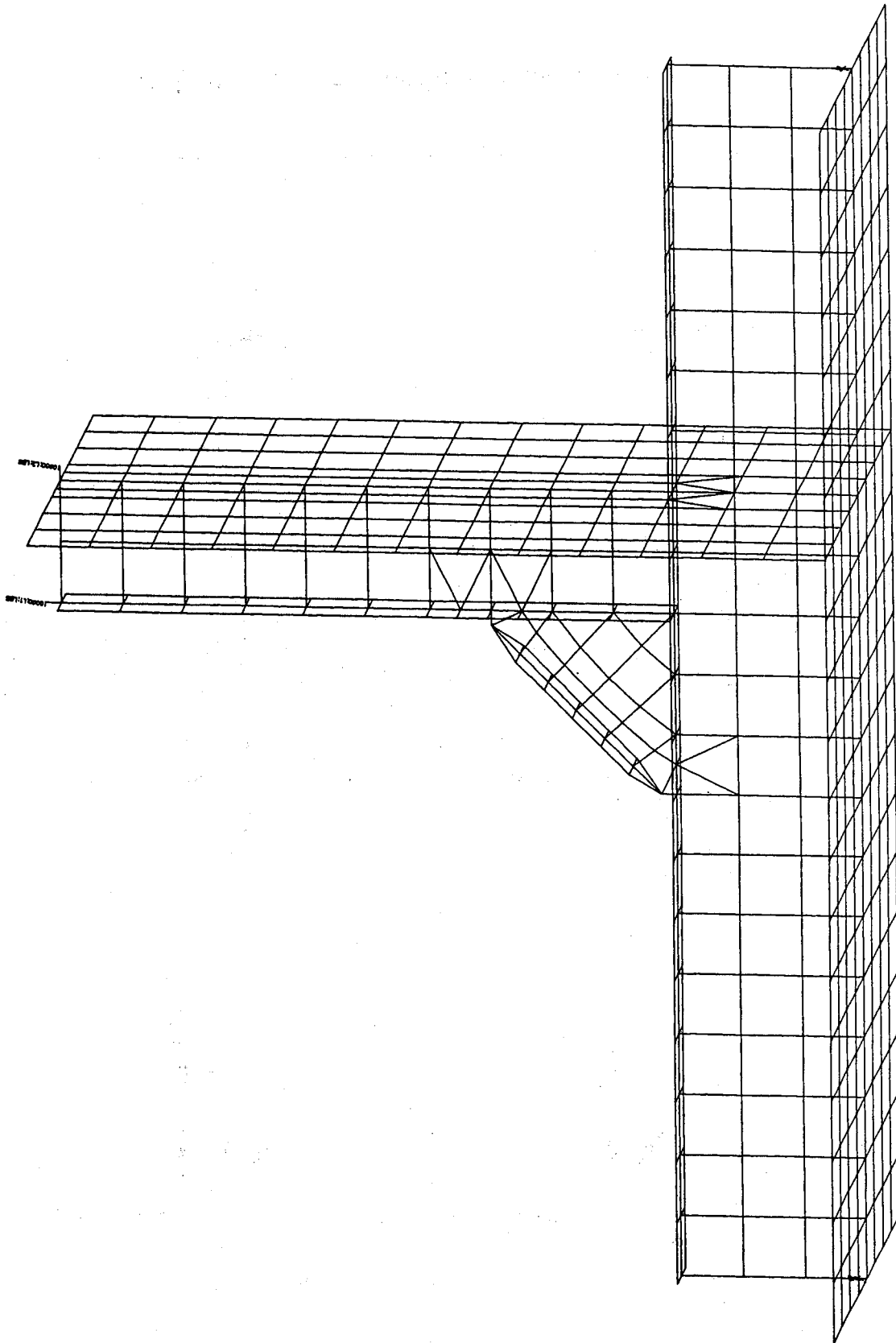
Figure A-18 FEA model of beam bracket
