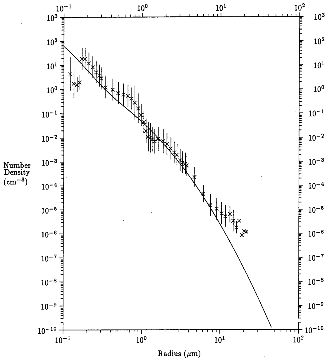
Figure 4. Maritime aerosol, 70 percent relative humidity. Measured and modeled particle size distribution for a maritime aerosol from the Meppen 80 test. The solid line represents the theoretical size distribution that has been normalized to the particle surface area. The vertical bars represent \pm 1 standard deviation about the data points.
