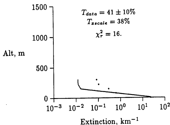
Figure 41. Sprekensehl block 735 and XSCALE profile.
