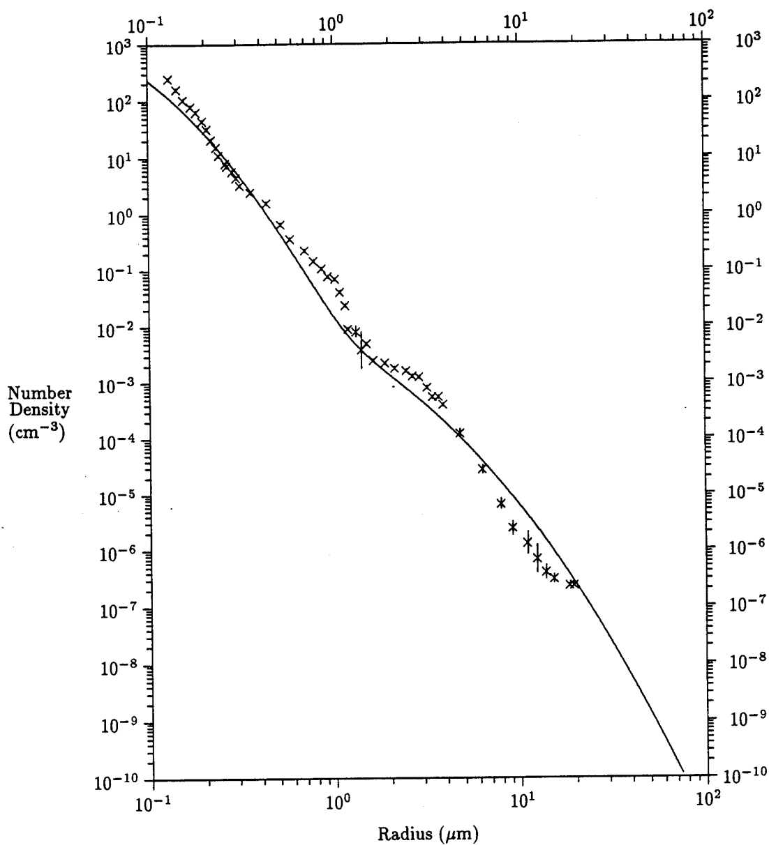
Figure 1. Rural aerosol, 90 percent relative humidity. Measured and modeled particle size distribution for a rural aerosol from the Cardington test. The solid line represents the theoretical size distribution that has been normalized to the particle surface area. The vertical bars represent \pm 1 standard deviation about the data points.
