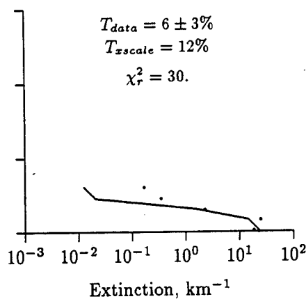
Figure 41. Sprekensehl block 735 and XSCALE profile.
