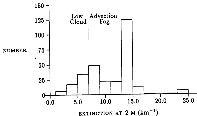
Figure 16. Frequency distribution of the surface extinction in steps of 2 \text{ km}^{-1} for the low cloud/fog cases.
