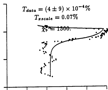
Figure 36. Cardington flight 27 and XSCALE profile.
