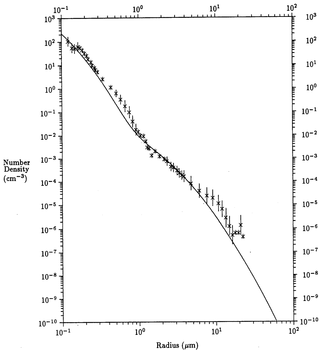
Figure 3. Rural aerosol, 70 percent relative humidity. Measured and modeled particle size distribution for a rural aerosol from the Meppen 80 test. The solid line represents the theoretical size distribution that has been normalized to the particle surface area. The vertical bars represent \pm 1 standard deviation about the data points.
