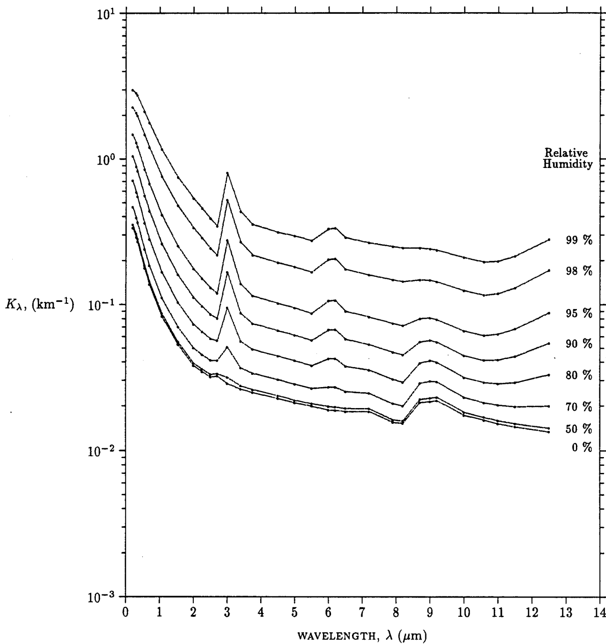
Figure 7. Urban extinction as a function of wavelength and relative humidity for a constant density of 20,000 particles/cm 3 . Semilog scale used.
