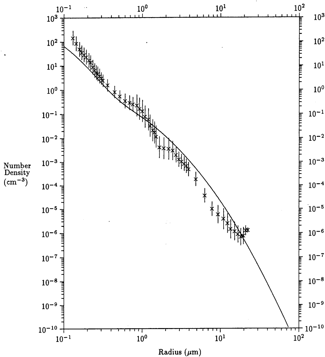
Figure 2. Maritime aerosol, 90 percent relative humidity. Measured and modeled particle size distribution for a maritime aerosol from the Cardington test. The solid line represents the theoretical size distribution that has been normalized to the particle surface area. The vertical bars represent \pm 1 standard deviation about the data points.
