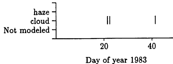
Figure 29. Cardington balloon flight data times. The y-axis denotes the type of profile, or an unsuitable data block.
