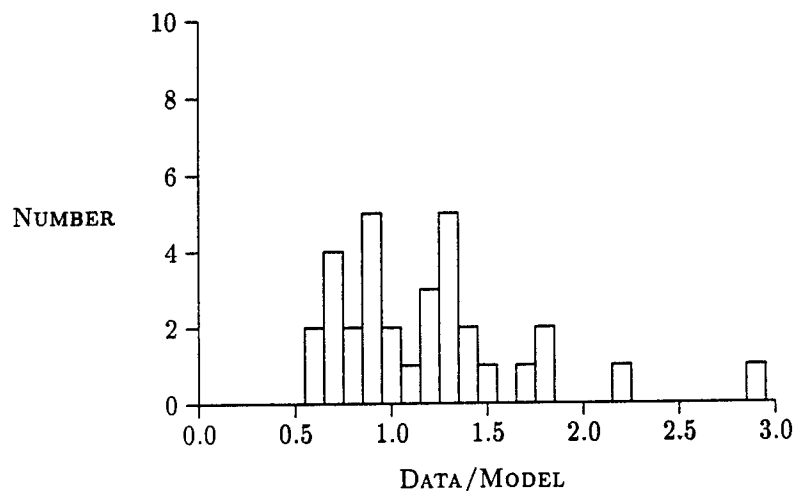
Figure 13. Data-to-model extinction ratio at 0.55 \mu\text{m} . Frequency distribution of the ratios of 33 profiles. The data-to-model ratio of each profile is the average of the ratios at each altitude of measurement.
