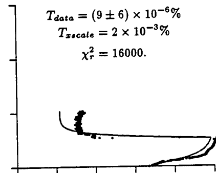
Figure 34. Meppen flight 7 and XSCALE profile.
