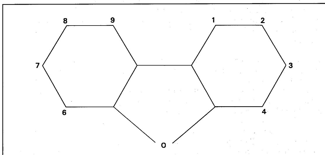
Figure 2. Polychlorinated dibenzofurans (PCDFs); chlorine atoms are substituted at one or more of the numbered locations on the molecule
