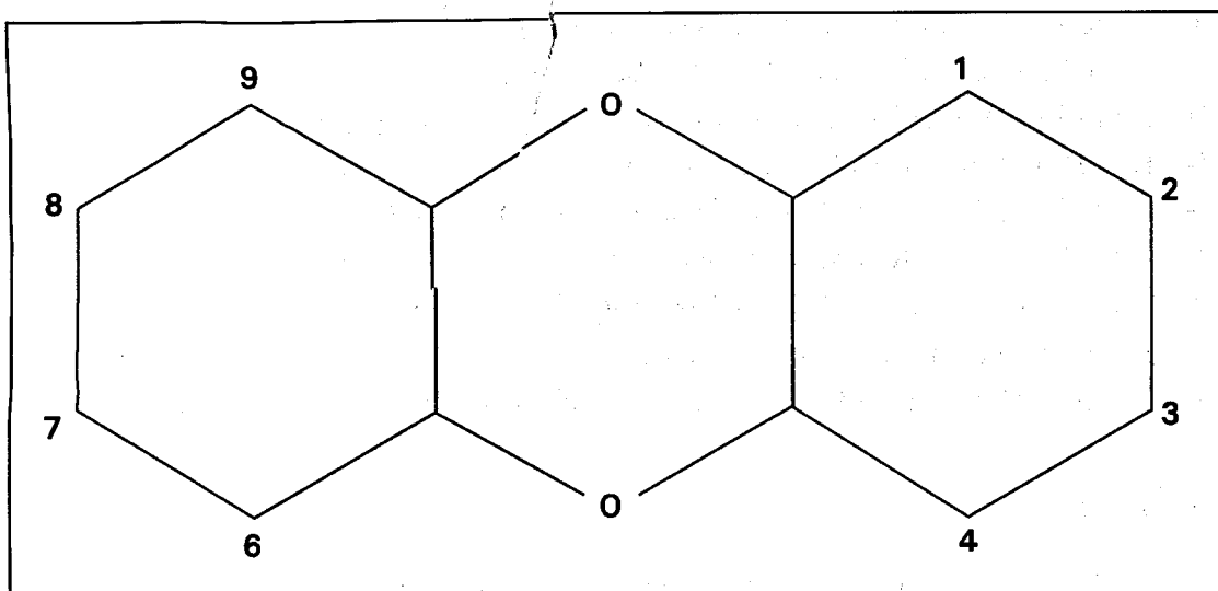
Figure 1. Polychlorinated dibenzo-p-dioxins (PCDDs); chlorine atoms are substituted at one or more of the numbered locations on the molecule
