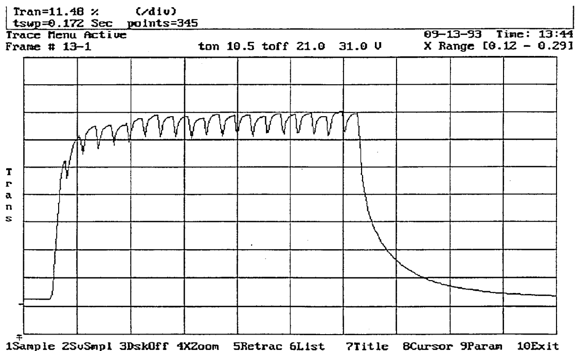
FIGURE 9. Electro-optic performance of PDLC containing 71% of liquid crystal TL 212 in standard polymer mix.
