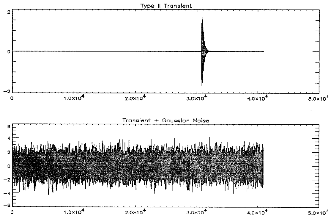
Figure 14. A ringing transient signal (top) with noise added to it (bottom)
