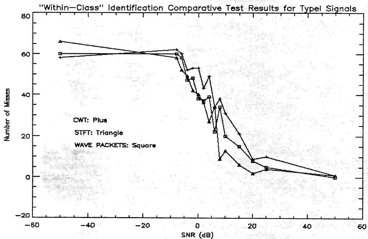
Figure 22. "Within-Class" Identification Results for Impulsive Transients (Type I)
