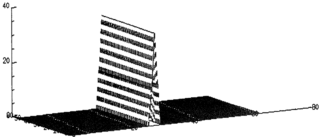
Figure 2. chirp(0,0,20) and its STFT
