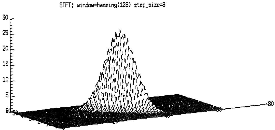
Figure 3. chirp(1,20,0) and its STFT
