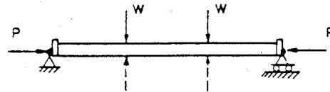
(b) Loading
