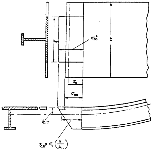
Figure 14.7 Use of transformed section to represent combined stiffener-and-plate as an equivalent elastic beam column.
