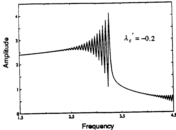
FIGURE 6A. NUMERICAL SIMULATION OF EQUATIONS (5.3). \lambda_c' = -0.1, -0.2 .
