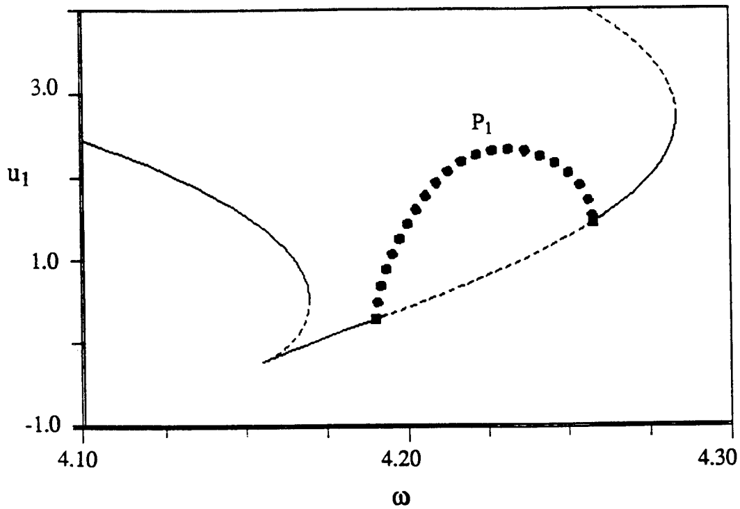
Fig. 10: Response amplitude for the limit cycle solution for u_1 as a function of the excitation frequency; Q_1 = 10.0 , Q_2 = 0.0 , c = 0.20 .
