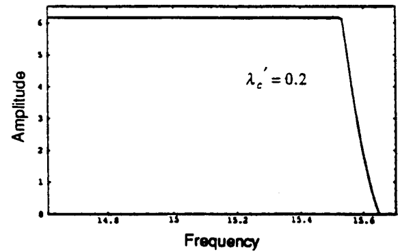
FIGURE 5B. AMPLITUDE RESPONSE. \lambda_c' = 0.1, 0.2 , \varepsilon = 0.1 .
