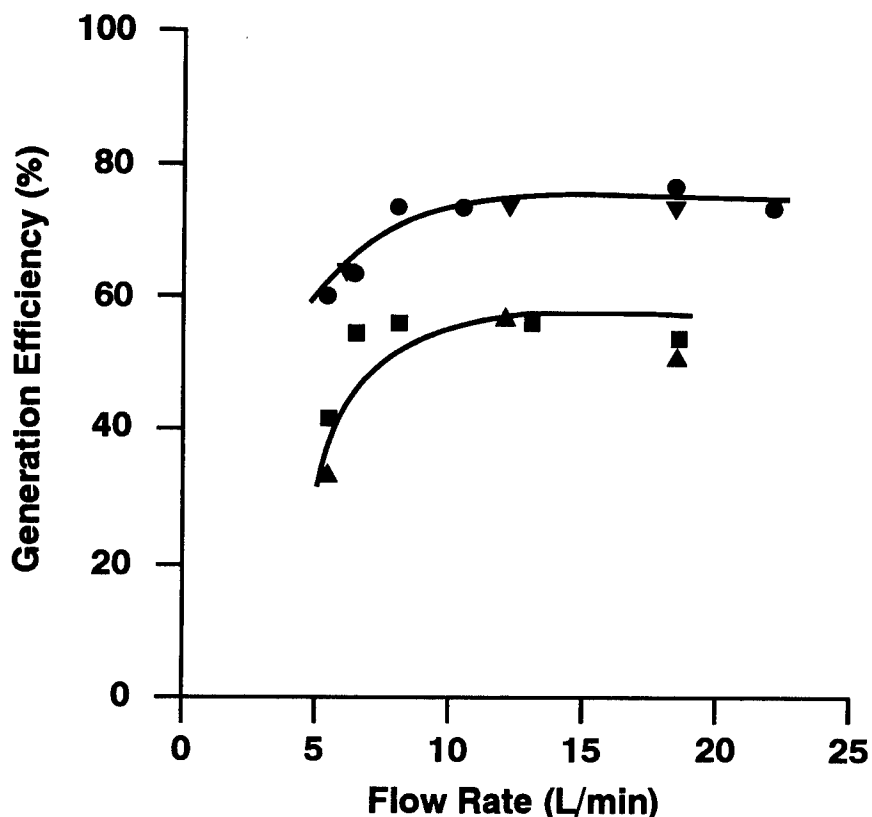
Figure 1. Dispersion efficiency as a function of flow rate in the TSI small-scale powder disperser for carbon fibers (●), 3-μm diameter polystyrene latex spheres (▼), talc (■), and alumina (▲).
