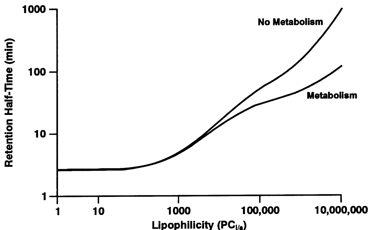
Figure 2. Simulated half-times of absorption of organic solutes in the airway mucosa as a function of their lipid/aqueous partition coefficient, following a transient exposure. Also indicated is the hypothetical influence on airway clearance by a constant activity metabolism within the epithelium.
