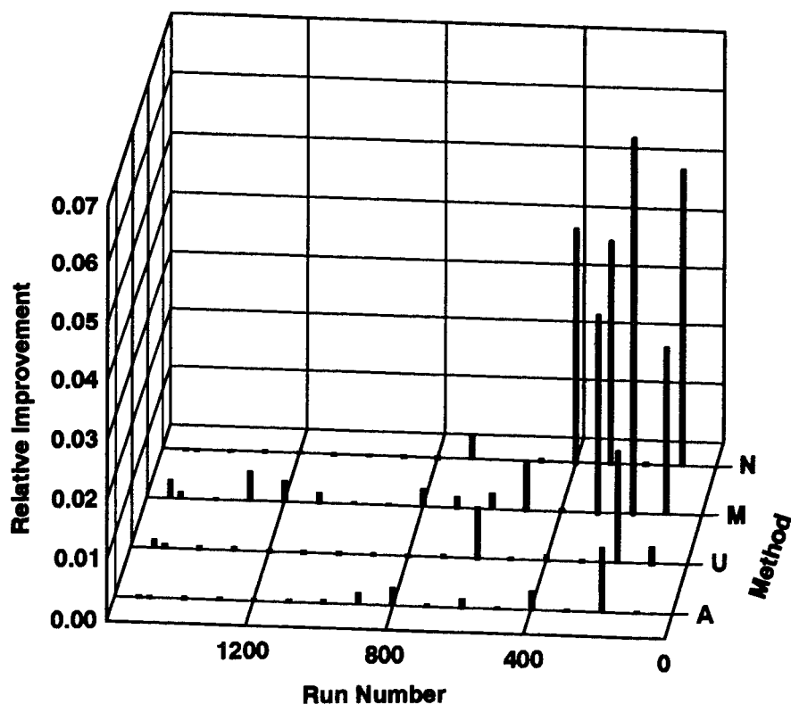
Figure 2. Improvement in the goodness of fit of the model as a function of the run number and the method of modification of the parameters. Improvement is defined as the difference between the previous best value and the new best value divided by the previous best value. Methods used are indicated by A for average crossover, U for uniform crossover, M for mutation, and N for changes in parameters made directly by the investigator. Values plotted are mean and standard deviation for each group of 100 runs.
