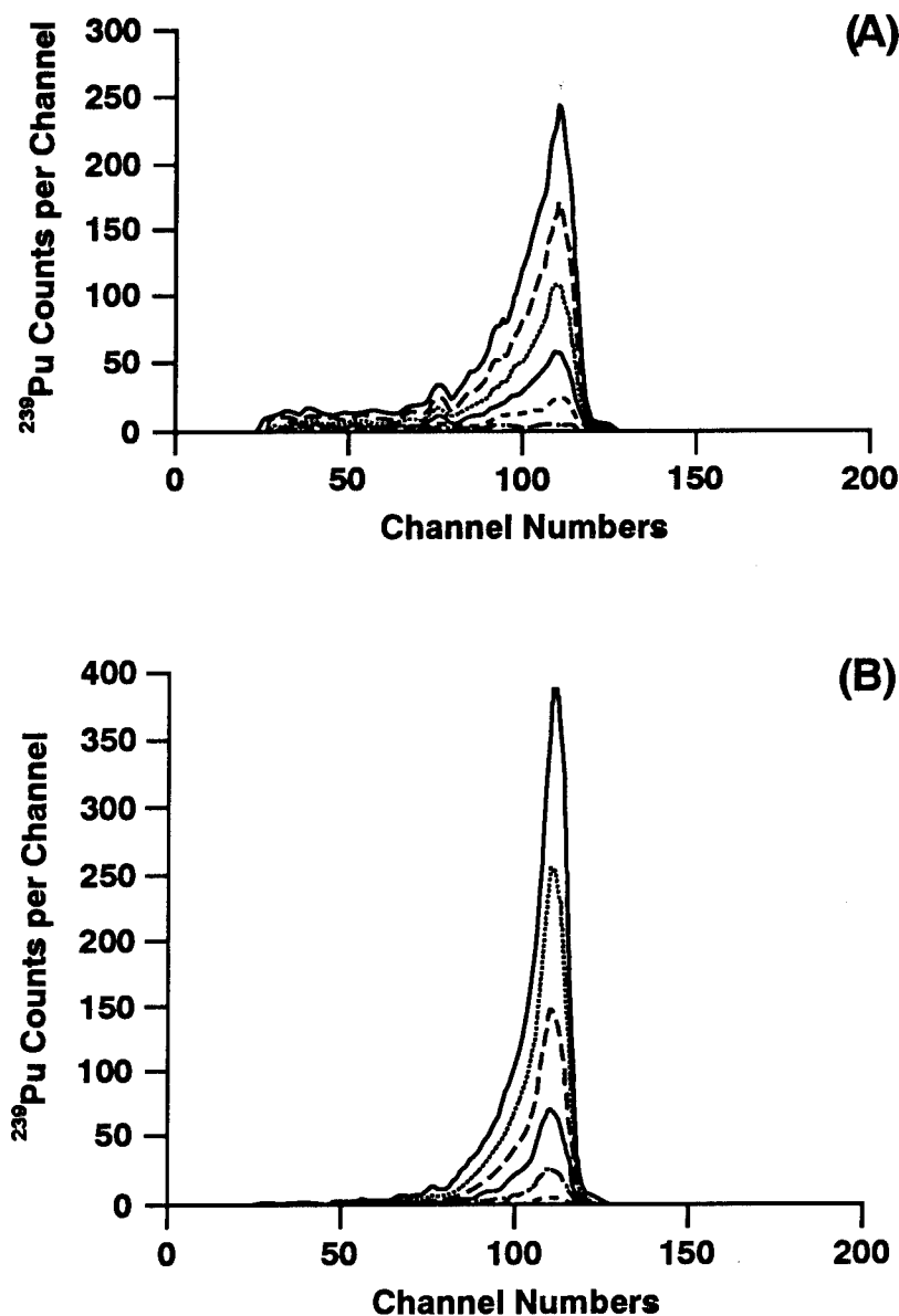
Figure 1. Alpha energy spectra demonstrating that energy resolution is (A) poorer when ^{239}\text{Pu} is collected on a clean Versapor 3000 filter, than (B) when collected on a salt-laden (14.6 mg) filter from WIPP.
