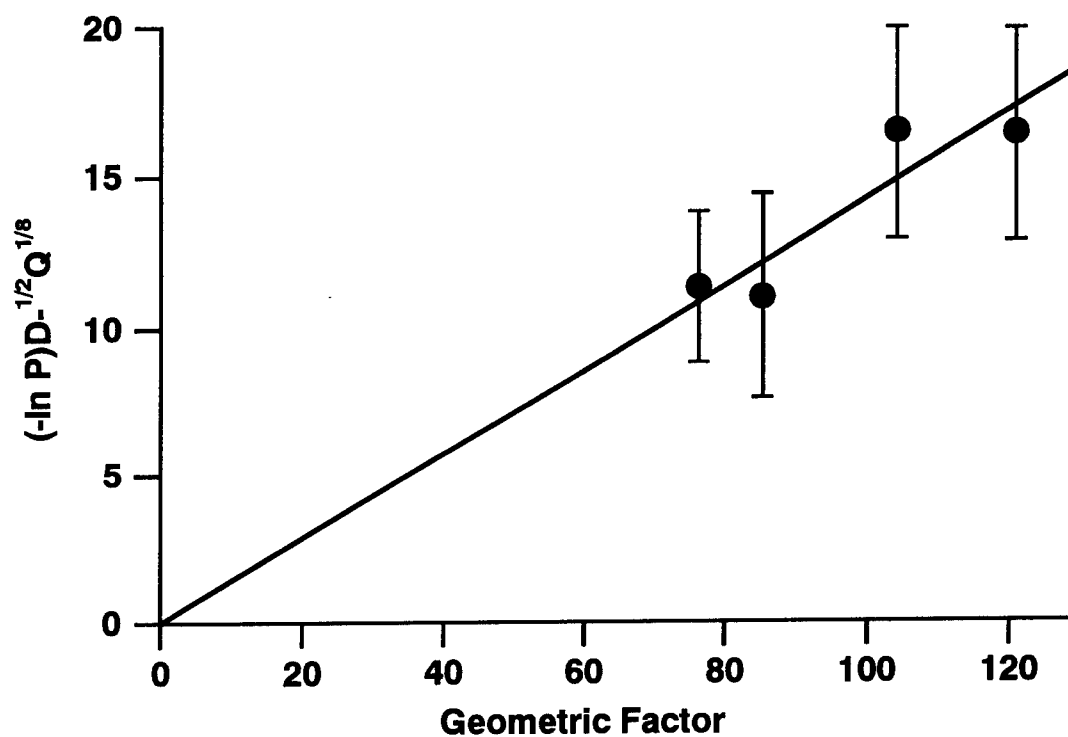
Figure 1. Correlation of the nasal deposition of ultrafine particles with the measured airway geometric factor (Mean \pm S.D.).
