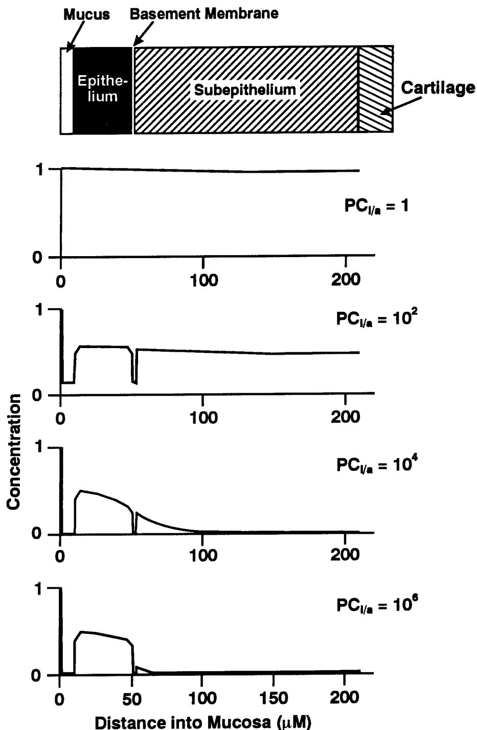
Figure 1. The model of the bronchial mucosa and four simulated concentration profiles of toxicants with different lipophilicities. PC_{l/a} indicates the lipid/aqueous partition coefficient of the toxicants. The concentration profiles are shown at the respective half-times of clearance of the toxicants following a transient exposure.
