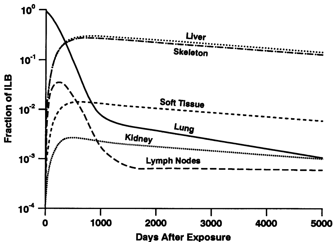
Figure 1. Pu distribution in a Beagle dog after inhalation of ^{238}\text{PuO}_2 . Results obtained from a materials balance simulation model fitted to Pu activity measurements in organs at death and in periodically collected excreta.
