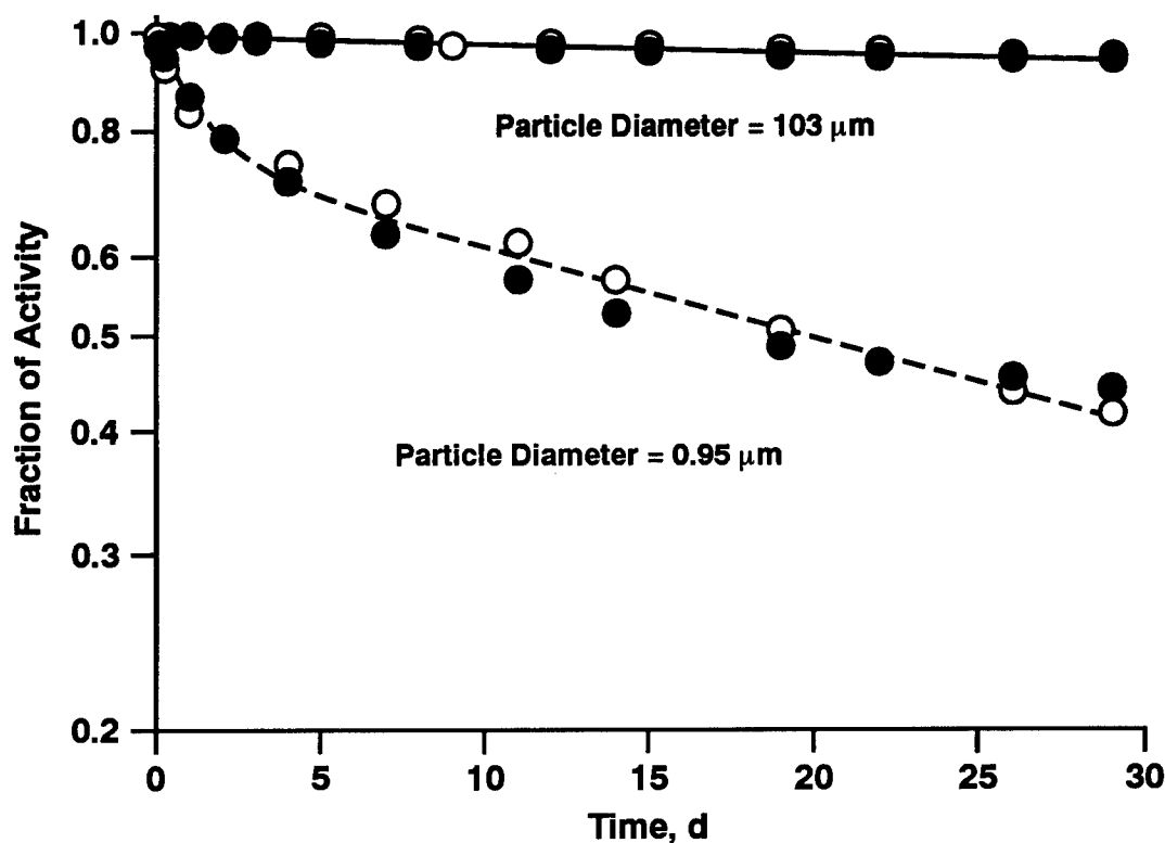
Figure 2. Retention curves of ^3\text{H} in a serum ultrafiltrate solvent for the coarse and fine titanium tritide powders. Open and closed circles represent the results for duplicate samples.
