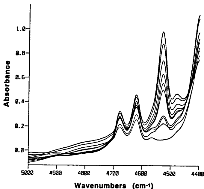
FIG. 3. FT-NIR spectra of the DGEBA/DEA concentration series. Epoxide concentration ranges from pure DGEBA (top) to pure DGEBA/DEA adduct (bottom). The 40% (w/w) DGEBA/DEA is omitted due to limitations in computer software.
