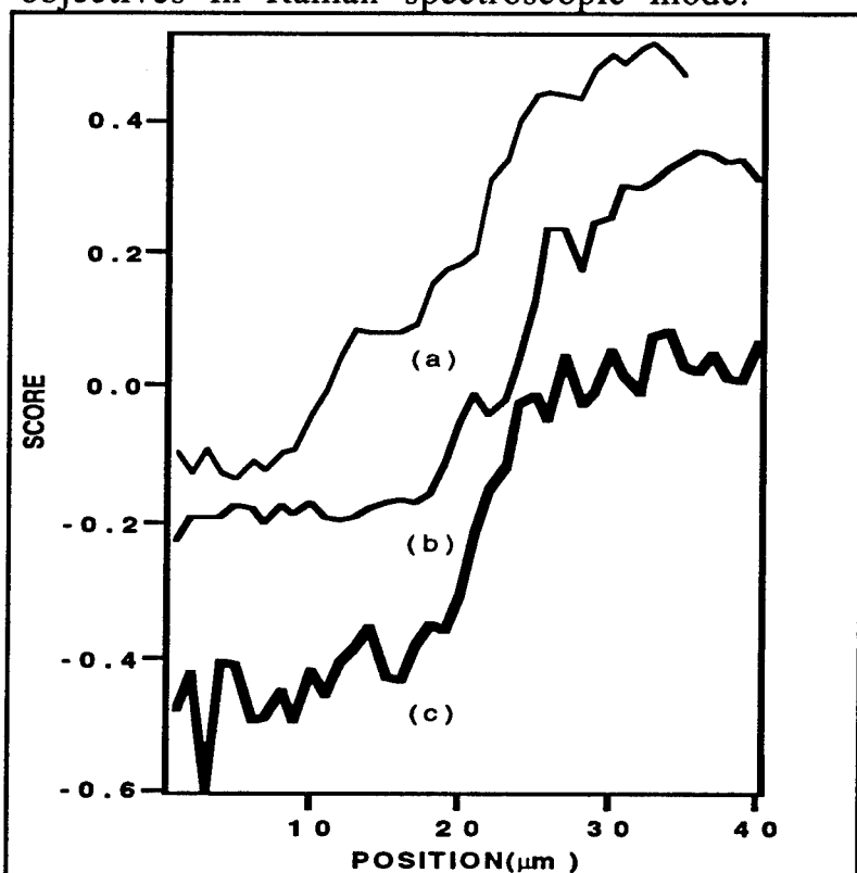
Figure 16: PCA of an interface crossing detected with Raman scattering using the USC microRaman with a (a) 10X objective, (b) 20X objective, and (c) 52X objective
