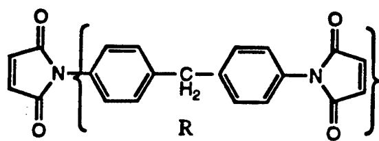
Component A
