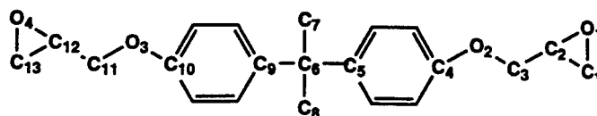
FIG. 8. Atomic labeling of DGEBA.
