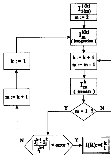
Figure 17 Flowchart for the method of averages
