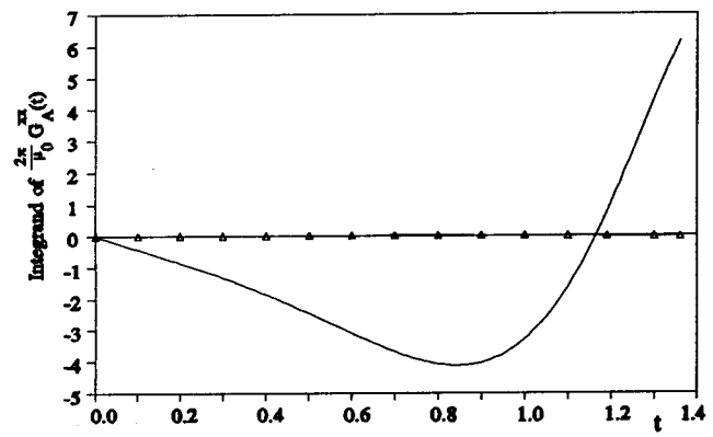
Figure 16 Integrand of (2\pi/\mu_0)G_A^{xx} (real (—) and imaginary (—Δ—Δ—Δ—)) after substitution.
