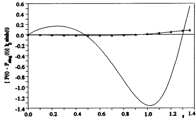
Figure 15 2\pi\epsilon_0 G_V difference term integrand (real (—) and imaginary (—Δ—Δ—Δ—)) after substitution \lambda = k_0 \cosh t .
