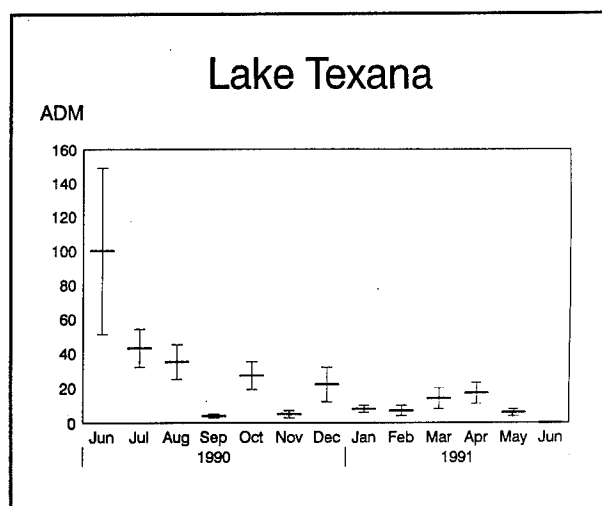
Figure 2. Average daily movement (ADM) ( \text{m} \cdot \text{d}^{-1} ) of triploid grass carp stocked in 1990, Lake Texana, Texas. Error bars represent standard errors
