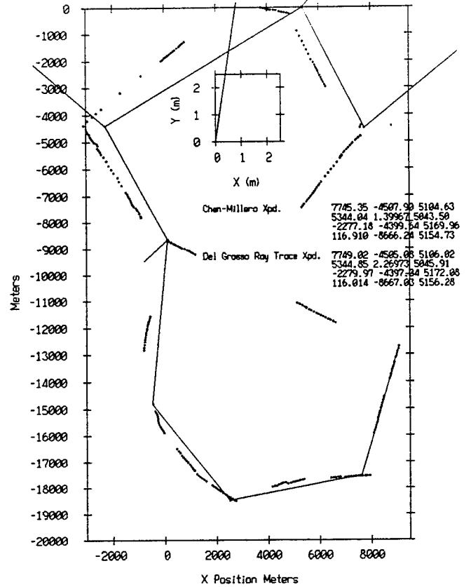
X-Y Directional Movement From Chen-Millero to Del Grosso Ray Trace Transponder Positions - VAST 1989
