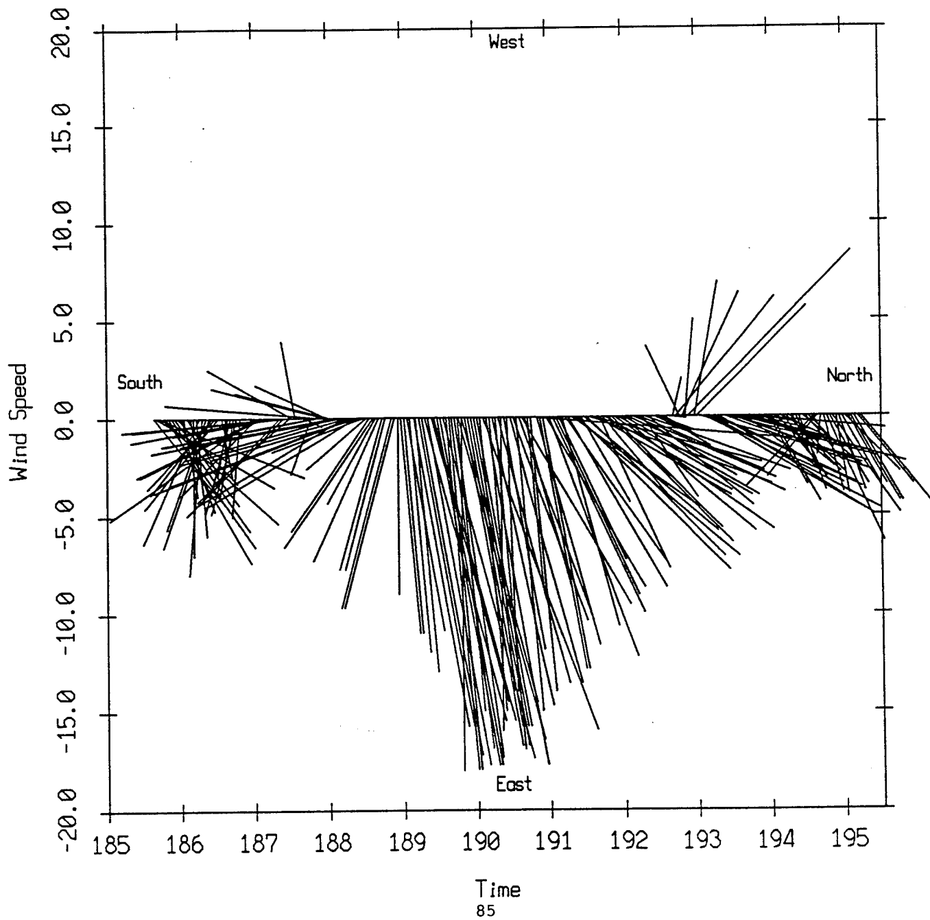
Figure 29C Wind Speed Vs. Time Day 185 -> Day 195
