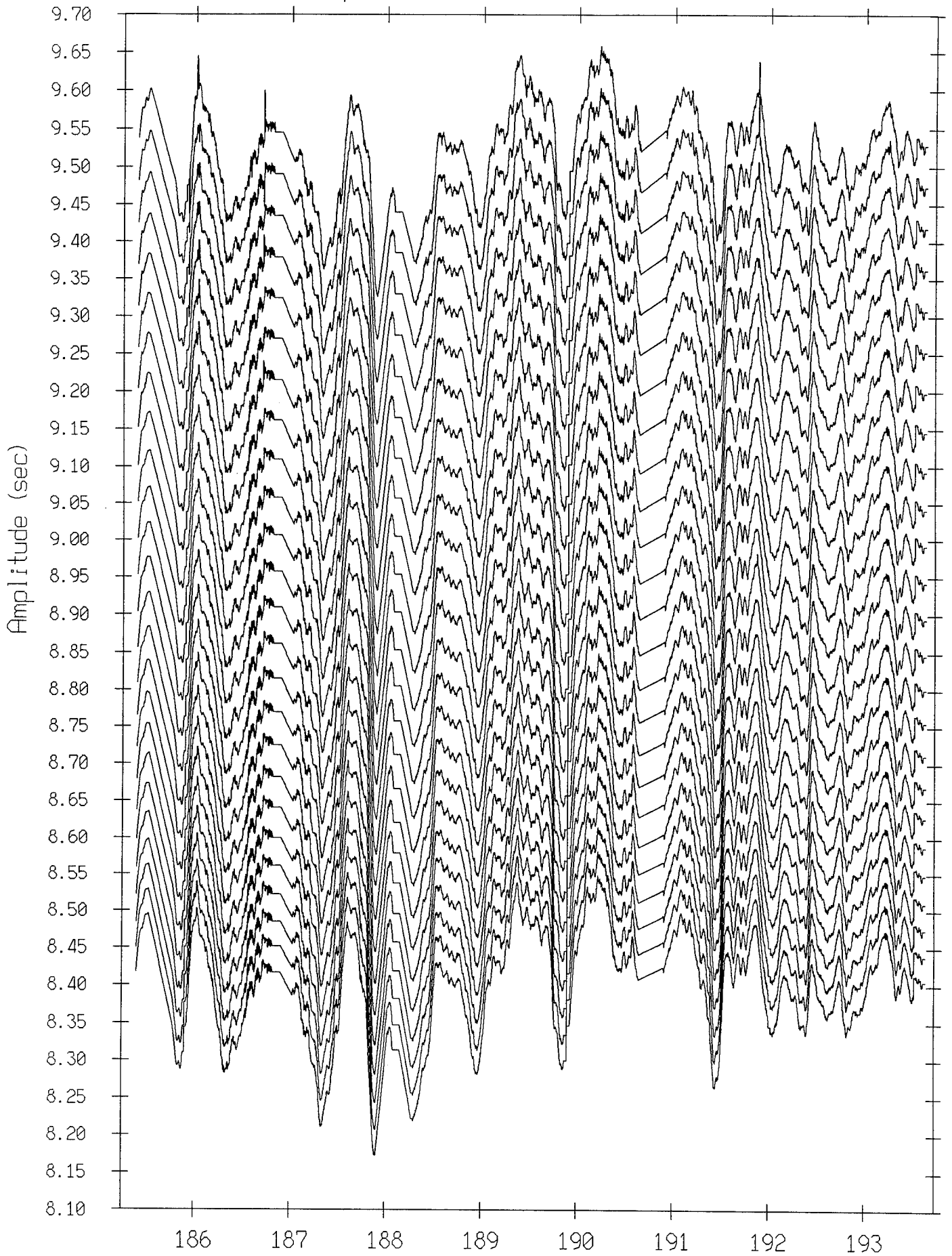
Figure 22D VAST MPL vertical array arrivals 11 th KHz transponder
