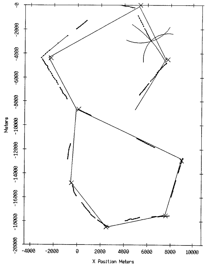
Transponder Positions (Figure 9b)
