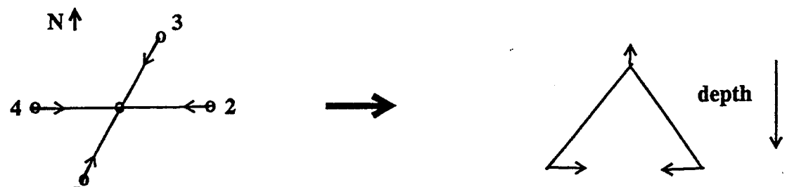
Figure 20.A.6 Inward/Outward transponder error raises/lowers depth of array 1-6m
