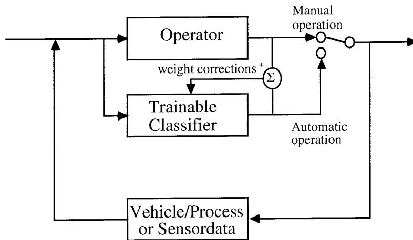
Figure 3.8 Identification Of Operator Characteristics By Observation
