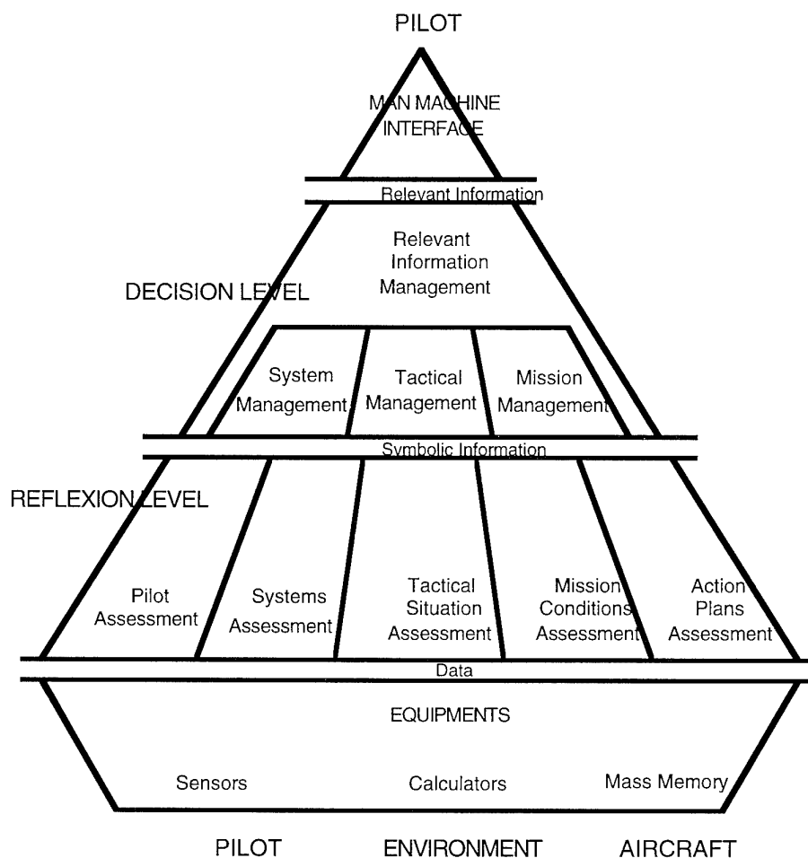
Figure 6.24 Copilote Electronique Architecture.
