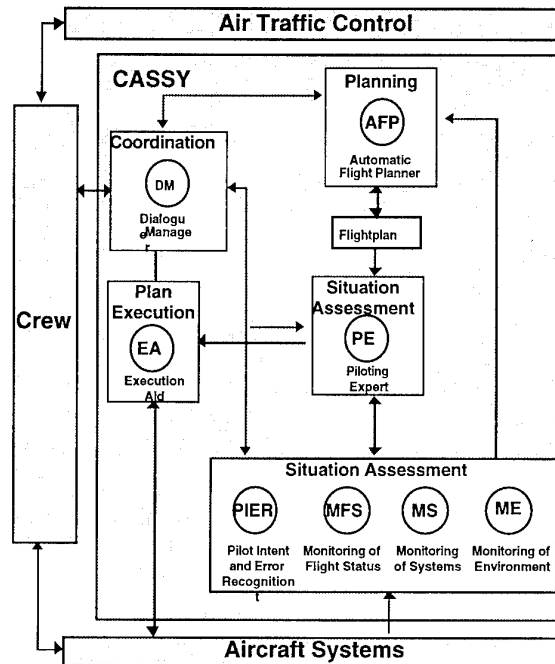
Figure 6.1 Functional Structure of CASSY
