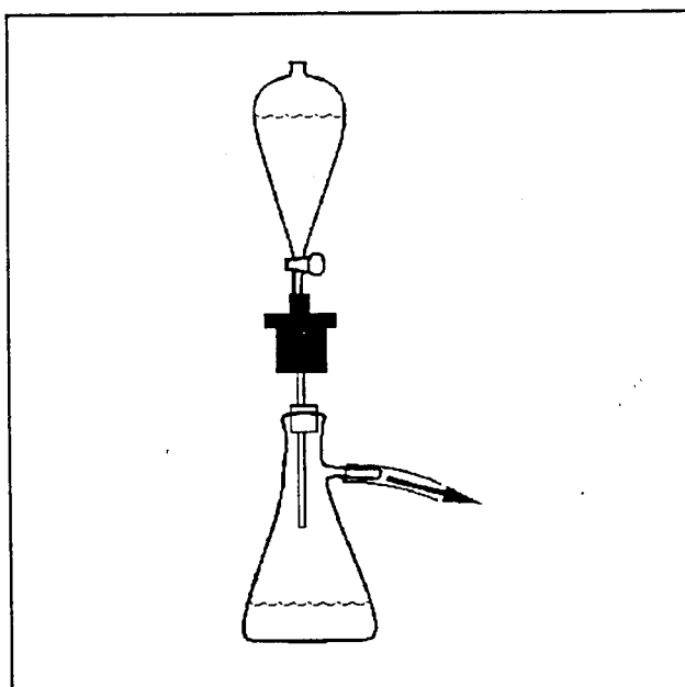
Figure 1. Vacuum Sample Collection Apparatus
