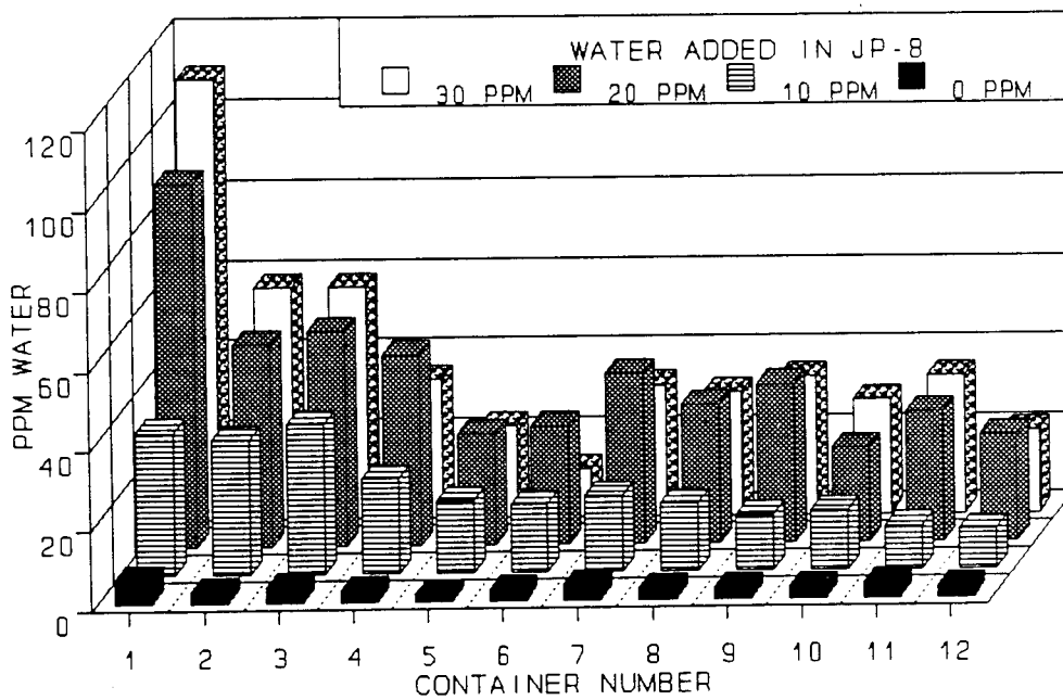
Figure 3. TMI Accumetric Measured PPM Water in JP-8
