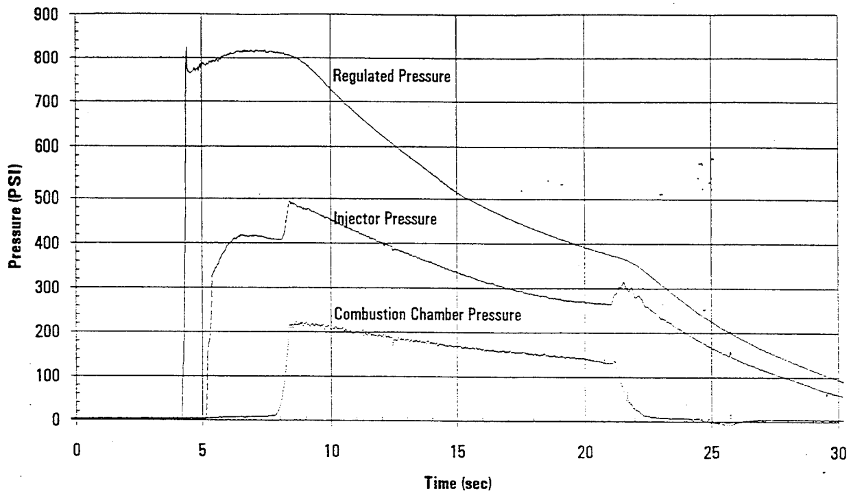
Fig 9 Static Test 2
