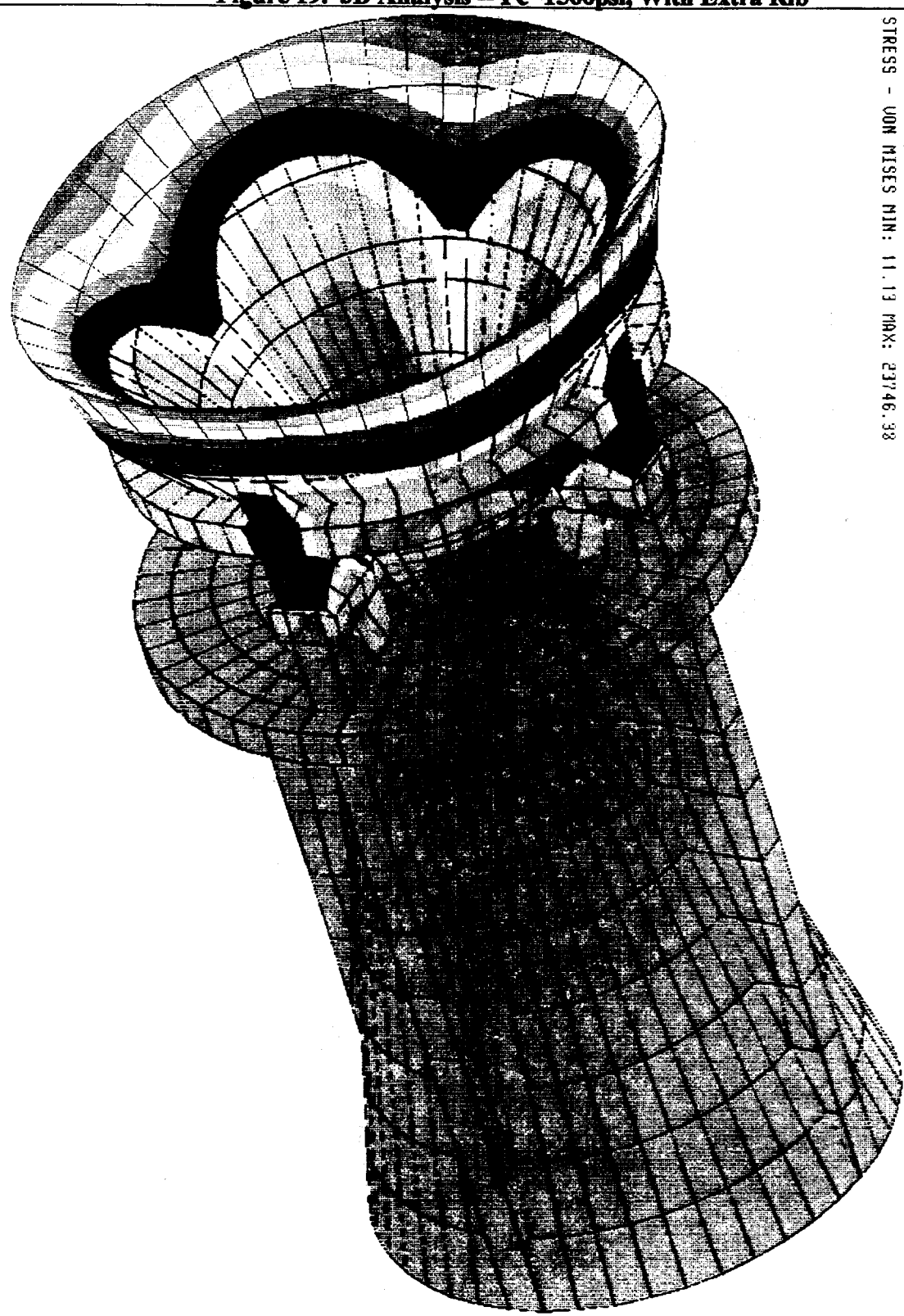
Figure 19. 3D Analysis -- PC=1500psi, With Extra Rib
