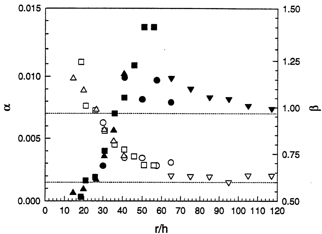
Figure 5: Pre-exponential factor, \alpha (filled symbols), and exponent, \beta (open symbols), vs. \bar{r} = r/h for 150 \mu\text{m} ( \nabla ), 250 \mu\text{m} ( \circ ), 300 \mu\text{m} ( \bullet ), and 400 \mu\text{m} ( \Delta ).
