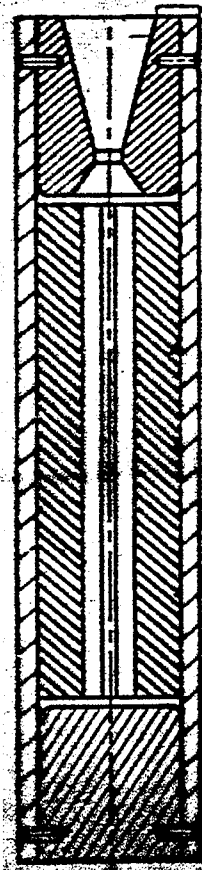
BOOSTER ASSEMBLY
