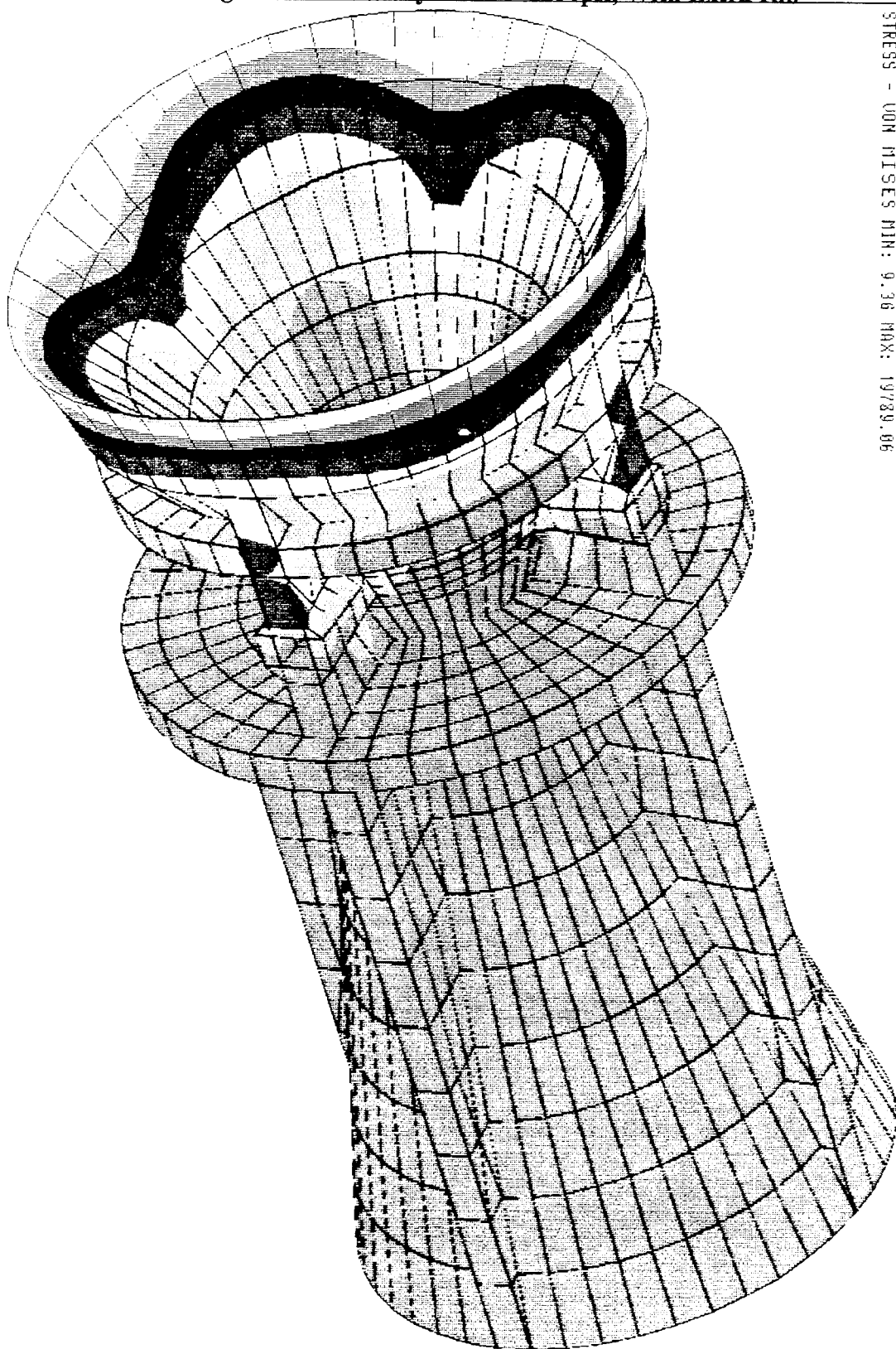
Figure 18. 3D Analysis - P_c=1250 psi, With Extra Rib
