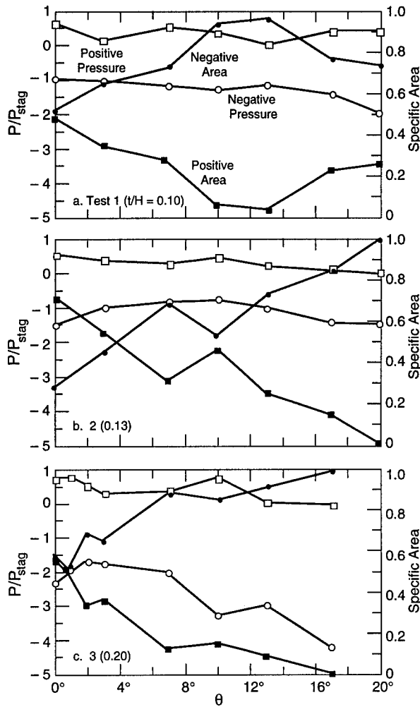
Figure 9. Areas of positive and negative pressure on the block's lower face, made nondimensional by the total block area. Also shown are the average pressures, made nondimensional with the stagnation pressure of the flow.
