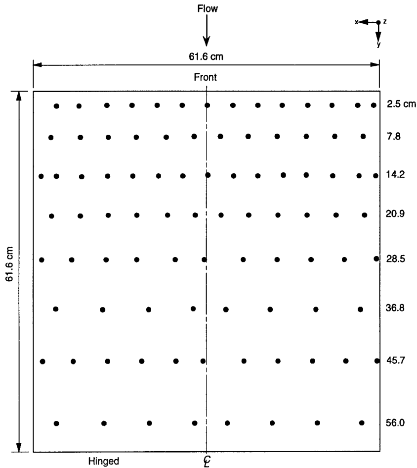
Figure 4. Tap locations. They were variably spaced in both the X and Y directions.
