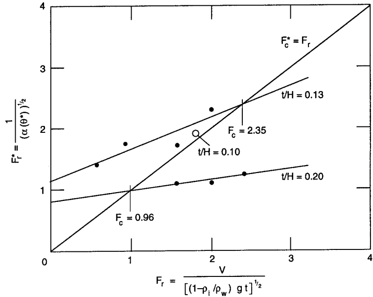
Figure 14. Froude criterion for block stability.
