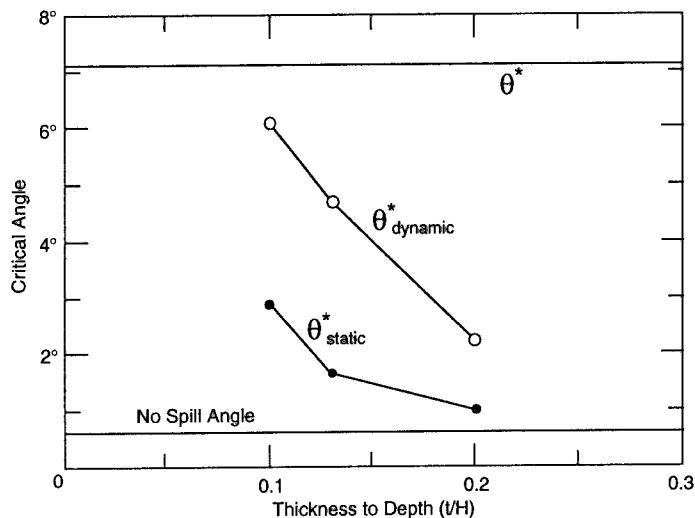
Figure 19. Angles at which the model ice floe achieves metastability.
