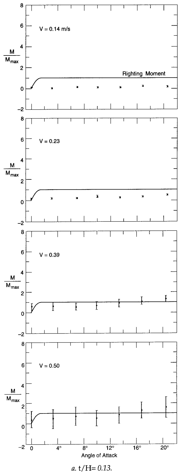
Figure 12. Nondimensional overturning moment vs. angle of attack.
