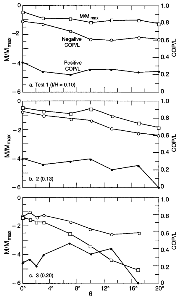
Figure 10. Center of negative and positive pressure divided by block length along with the total underturning moment, made nondimensional by the maximum hydrostatic righting moment (COP/L = 0 is the axis of rotation).
