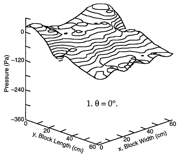
Figure 7. Typical pressure distribution surface plot. This is created by reading selected taps along one side of the block and generating a mirror image of the pressures on the opposite side. In this example V = 0.39 m/s, t/H = 0.13 and \theta = 0^\circ .
