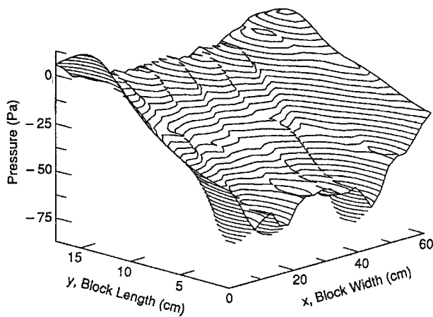
Figure 6. Surface plot showing a typical pressure distribution across the full width of our block during a symmetry check. Only the first three rows of taps were used; V = 0.35 m/s, t/H = 0.05 and \theta = 0^\circ .
