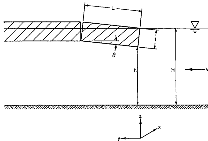
Figure 1. Underturning block problem.
