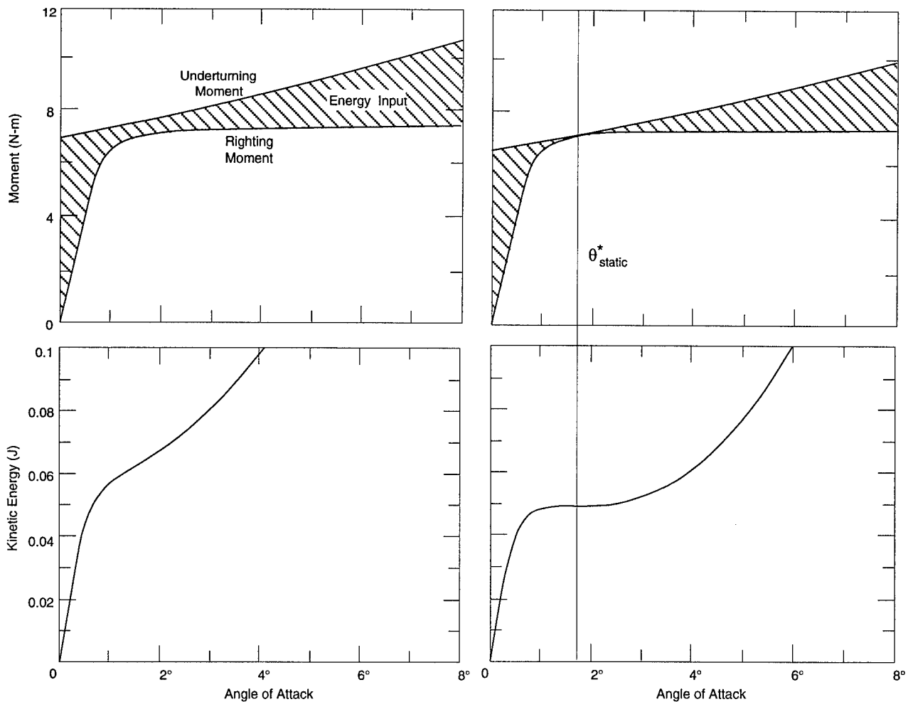
a. Unstable block at t/H = 0.13 and V = 0.55 m/s.
