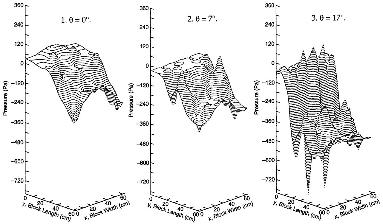
Figure 8 (cont'd). Representative pressure distributions from three tests. The block's trailing edge is at Y = 0 .
