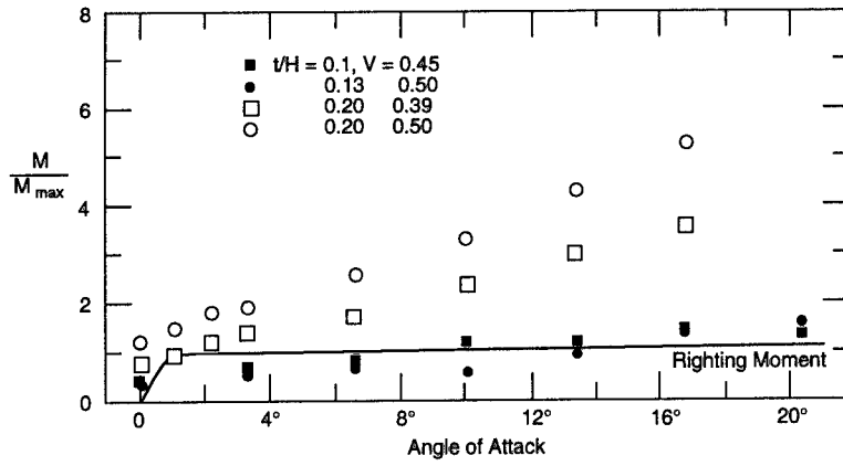
Figure 13. Nondimensional overturning moments vs. angle of attack for different t/H ratios at similar velocities.
