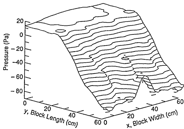
Figure 7. Typical pressure distribution surface plot. This is created by reading selected taps along one side of the block and generating a mirror image of the pressures on the opposite side. In this example V = 0.39 m/s, t/H = 0.13 and \theta = 0^\circ .
