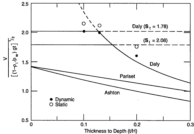
Figure 18. Comparison of calculated stability points with existing stability criteria.
