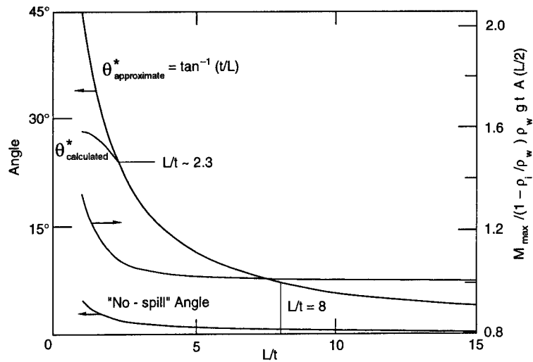
Figure 2. Hydrostatic righting moment. Both the calculated and approximate angle at which the maximum hydrostatic righting moment occurs are plotted vs. the block-length-to-thickness ratio. Our block L/t = 8 . Also shown is the previously used “no-spill” angle condition for block instability.
