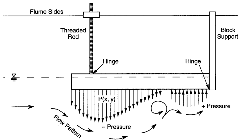
Figure 5. Block attached to the flume at the front by a threaded rod and at the rear by hinged supports. These held the block rigid during a test but still allowed the attack angle to be changed.
