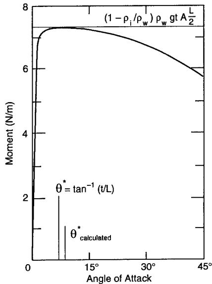
Figure 3. Calculated block hydrostatic righting moment for our particular block vs. angle of attack. Both the calculated and approximate angles of maximum righting moment are also shown. The horizontal line is the approximated maximum righting moment for our block.
