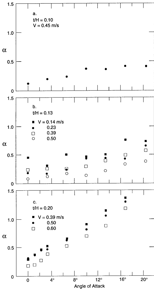
Figure 11. Nondimensional moment coefficient vs. angle of attack.
