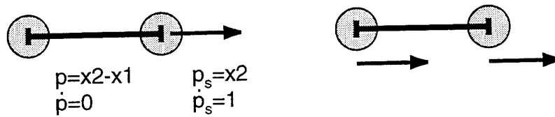
Figure 3.7: Two points are connected by a hard control constraining their distance. The right point is also pulled by a soft control. If the soft controls are computed independently, a non-optimal solution may be found, as shown on the left. The soft control may specify that the right point should move, but part of this motion might be removed by the constraints. As shown on the right, there is a solution that both satisfied the constraints and meets the desired values for the soft controls.
