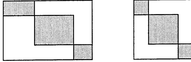
Figure 4.1: Sparsity patterns depicted by filling potentially non-zero elements with grey. Left: Since each object defines a few functions to contribute to the metric, and these functions depend only on the object's variables, the Jacobian will be block-sparse with a rectangular region for each object. Right: When the Jacobian is multiplied by its transpose, the blocks do not interact with each other, leading to independent squares along the diagonal of the matrix. This form of sparsity is called block-diagonal .
