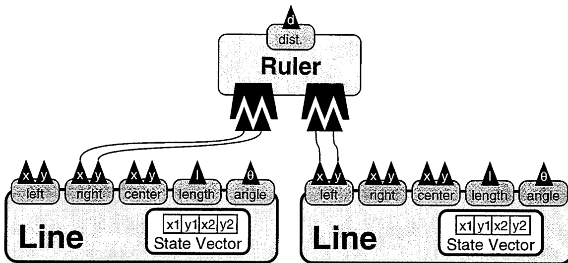
Figure 6.1: A schematic “wiring diagram” of two line segments with an attachment constraint between their endpoints. For the purposes of defining manipulations, these objects appear as a set of connectors awaiting controllers to be plugged into them.
