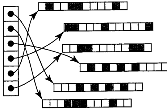
Figure 5.3: A half-sparse matrix representation store the matrix as a full vector of sparse vectors. Each entry in an array points to a sparse vector, depicted here by a sparsity pattern.
