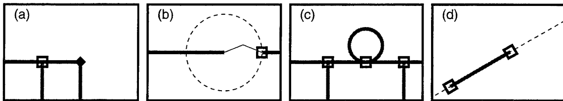
Figure 9.4: Snap-Dragging provides a basis for visual representation of constraints. The two basic constraints, point-on-object and point-to-point, are drawn as an empty square and a filled diamond (a) respectively. Other constraints are represented using the basic ones and alignment objects, for example, distance-between points (b), points-aligned (c), and orientation (d). Thin wedges as seen in (b), emphasize distance constraints. Color is used for constraint display when available.
