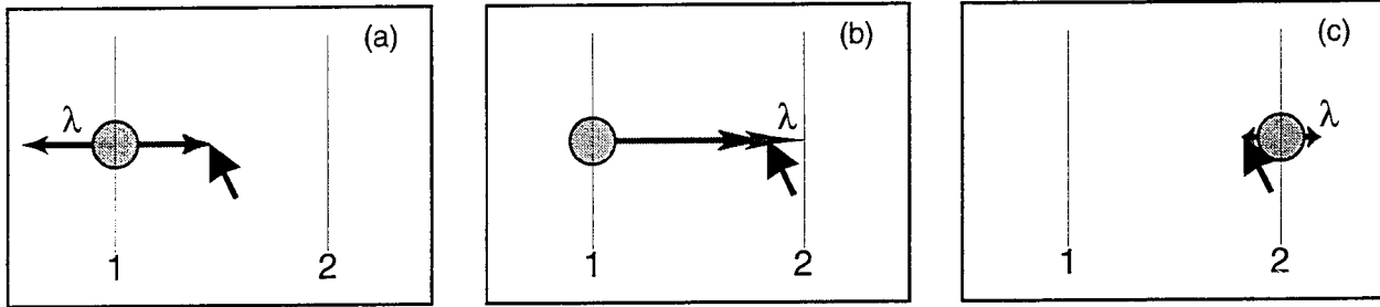
Figure 6.6: Clicking forces a value to be in a discrete set. The value, in this case the horizontal position of the circle, is constrained to have the value 1 or 2. Grey arrows represent the pull of the mouse control, black arrows represent the pull of the Click controller. Initially (a) it has value 1, so a GoTowards controller pulls to maintain this value as the mouse attempts to drag it with a pull labeled \lambda . At some point, the mouse pulls hard enough so that the pull vector's magnitude exceeds a limit value causing the controller to advance to the next click stop (b), causing the point to attain the next value in the set (c).
