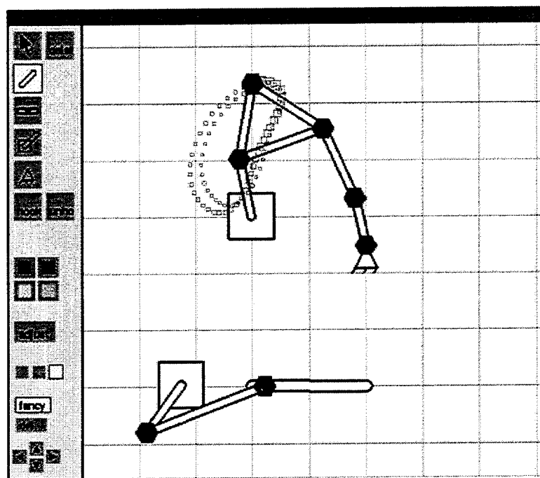
Figure 9.5: The Mechtoy application is specifically designed for drawing and animating planar linkage mechanisms. This picture shows a mechanism being animated, with smoke trails tracing the motion.
