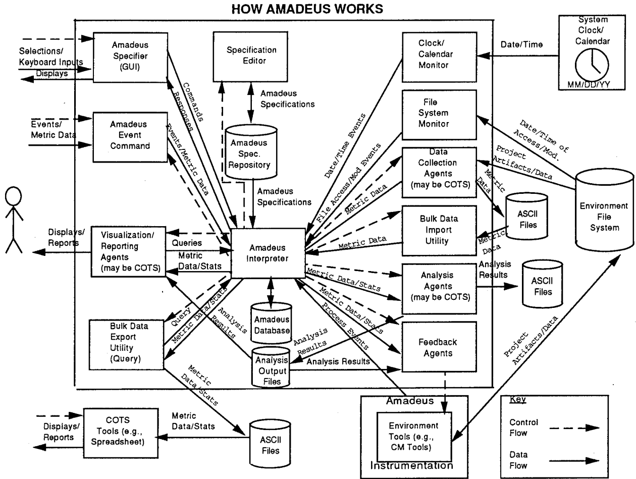
Figure 11: Amadeus Control and Data Flow
