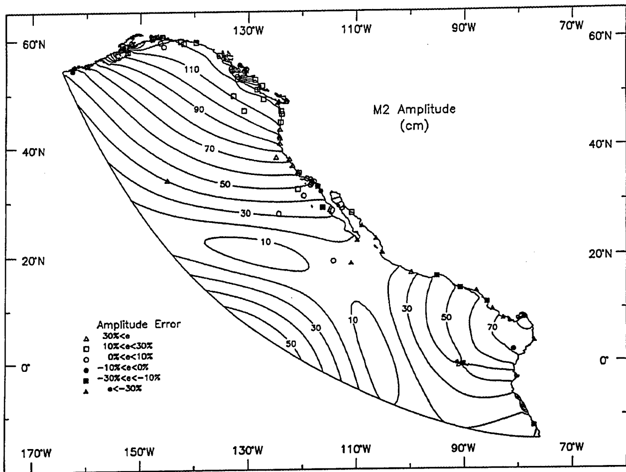
Figure 3. Computed contours for the M_2 amplitude (meters)
