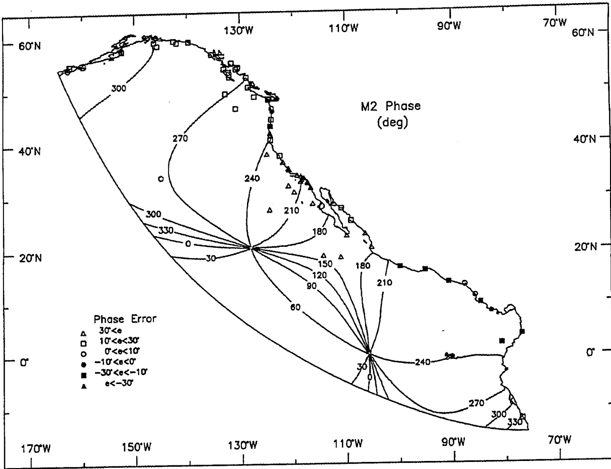
Figure 4. Computed contours for the M 2 Greenwich epoch G (degrees)
