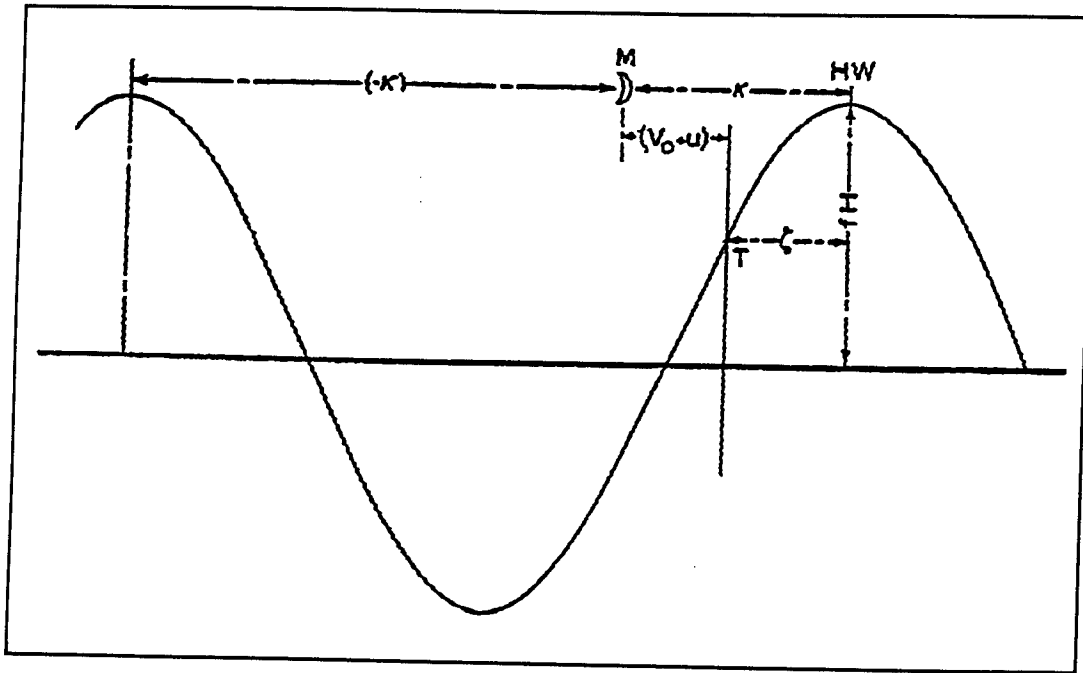
Figure 2. Tidal phase relationships (Schureman 1958)
