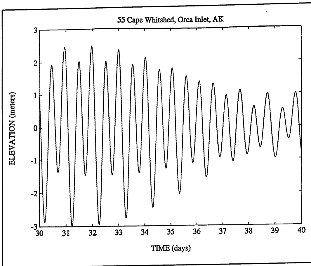
Figure 5. Manually computed equilibrium tidal elevation time series for Cape Whitshed, Alaska
