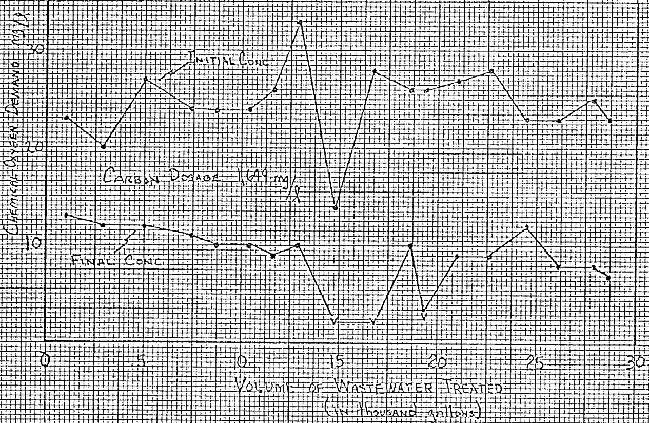
Figure 12. CHEMICAL OXYGEN DEMAND - mg/l
