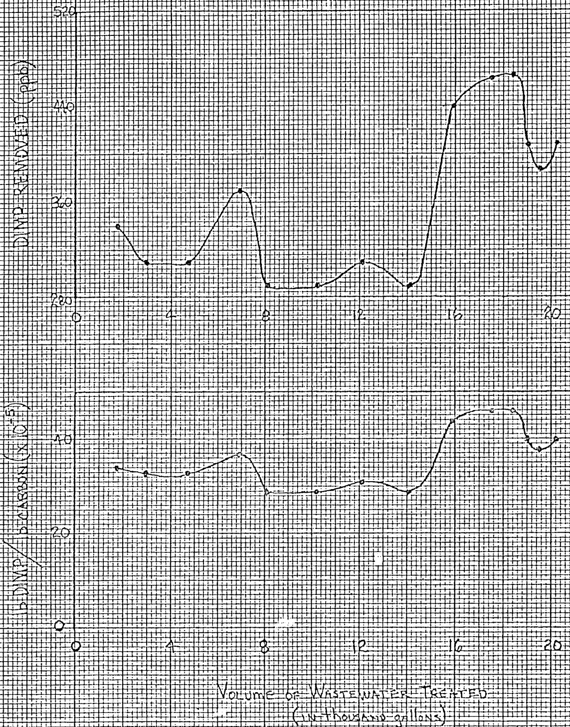
Figure 11. \frac{X}{M} for CARBON DOSEGE - 1,000 mg/l
