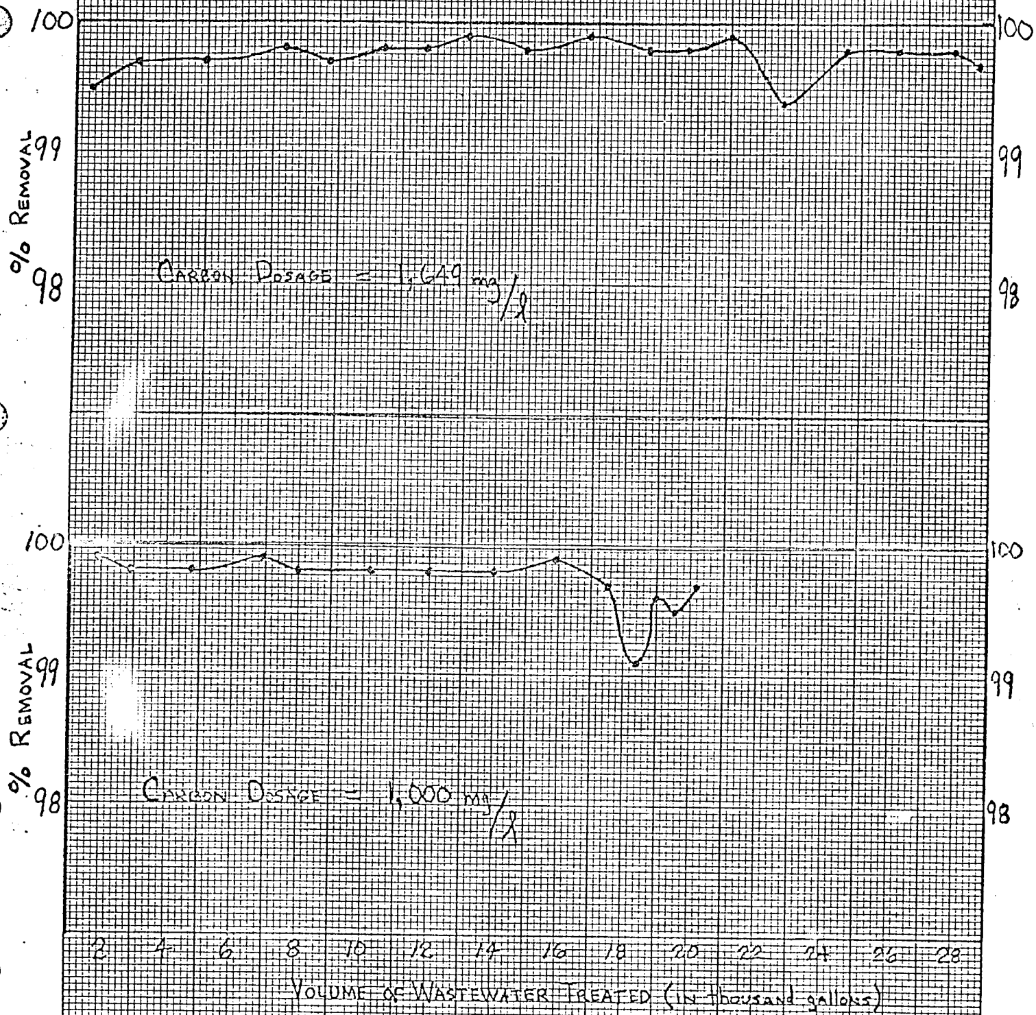
Figure 9. PER CENT DIMP REMOVAL
