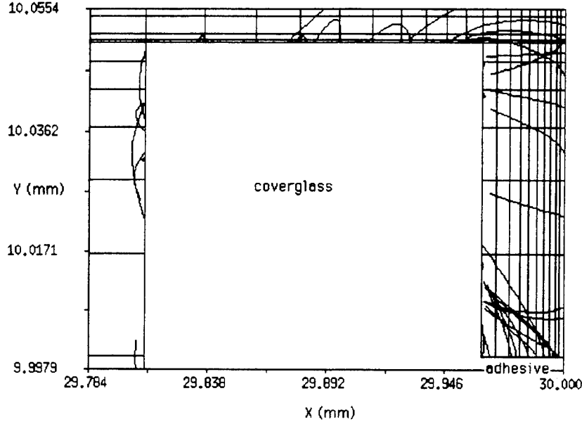
Figure 39: Electron trajectories for 50\mu\text{m} overhang; \beta V = 3 \times 10^5 \text{V}
