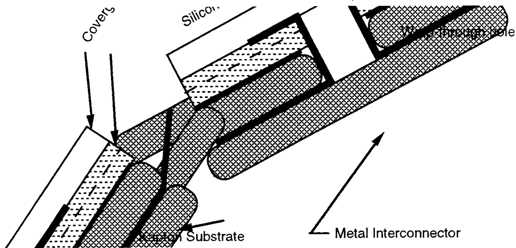
Figure 12: Schematic of a wrap-through-contact solar array
