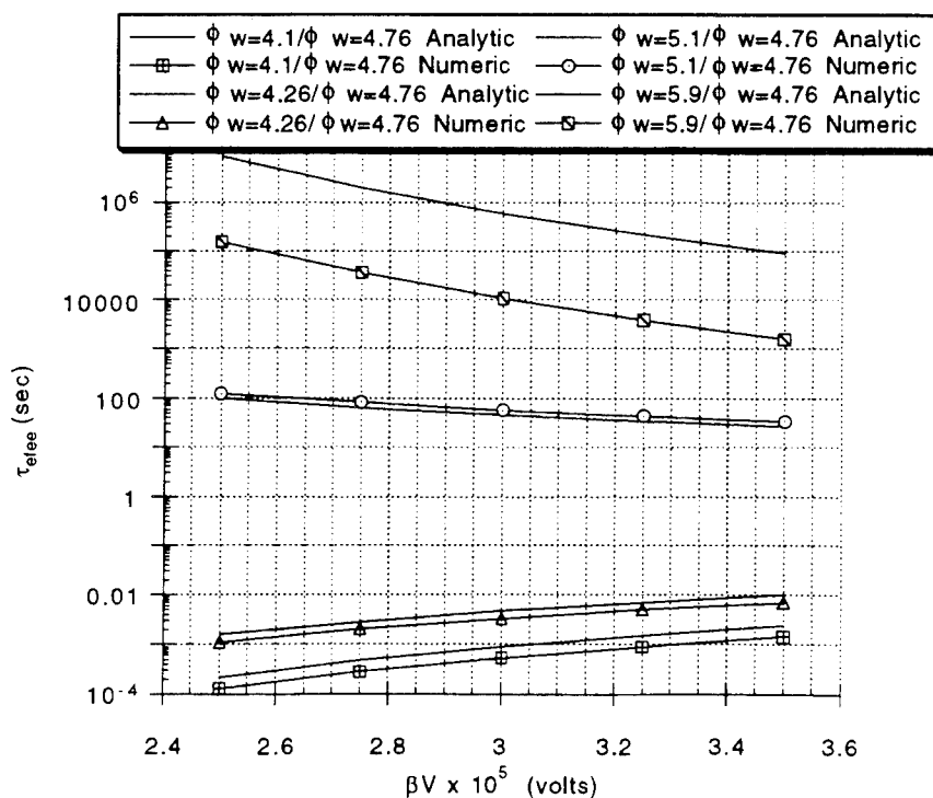
Figure 24: Analytic predictions and numerical results for \tau_{e,fee}/\tau_{e,fee}(\phi_w = 4.76 eV) versus \beta V
