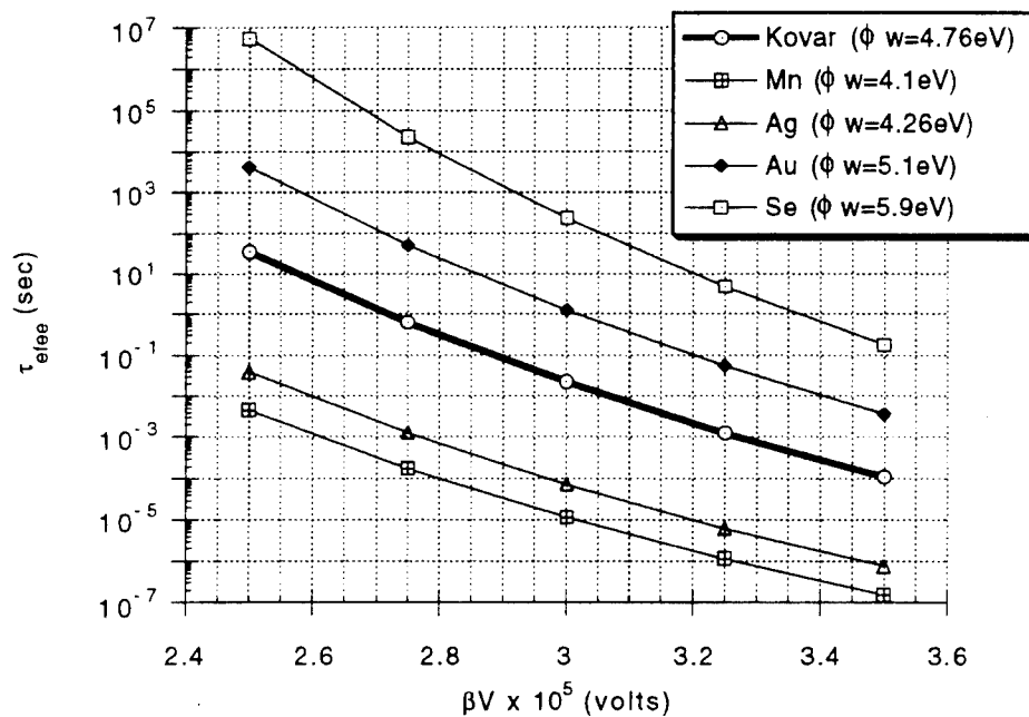
Figure 23: Enhanced field electron emission charging time, \tau_{e,fee} , versus \beta V for different work functions, \phi_w (eV)
