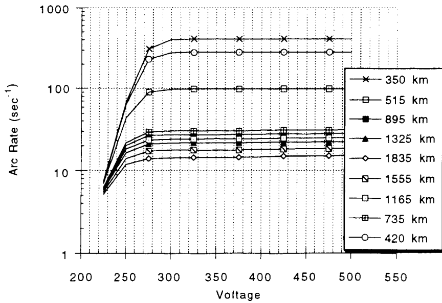
Figure 59: Complete arc rate predictions in the differentiating voltage range for APSA (#36)
