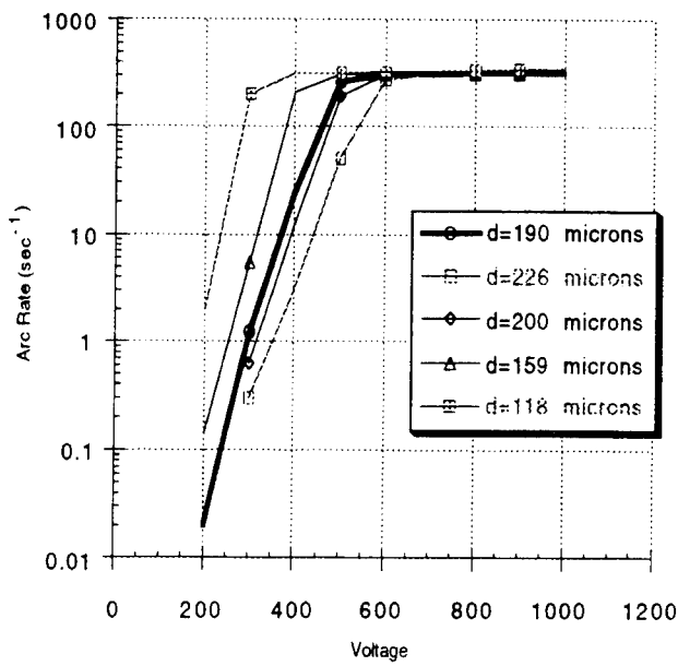
Figure 43: Analytic arc rates for varying dielectric thicknesses, d
