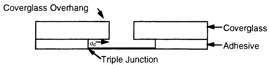
Figure 35: Model of coverglass overhang
