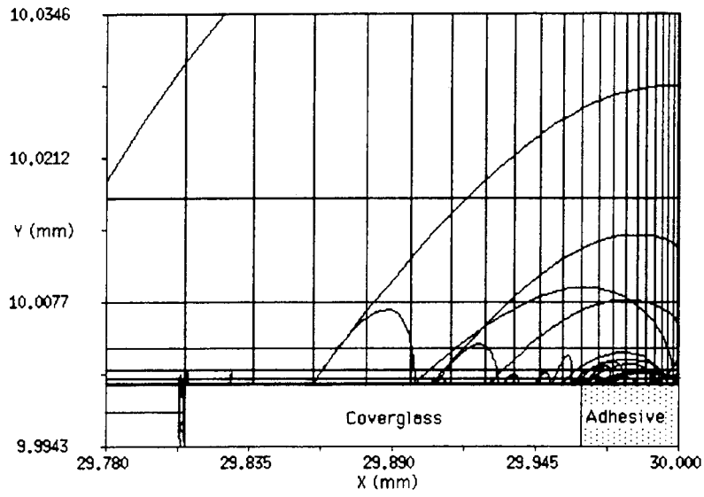
Figure 31: Electron trajectories for \epsilon_{d_1}/\epsilon_{d_2} = 2.7
