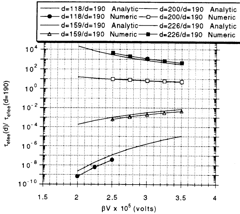
Figure 26: Analytic predictions and numerical results for \tau_{e_{f_{ee}}}(d)/\tau_{e_{f_{ee}}}(d=190) versus \beta V
