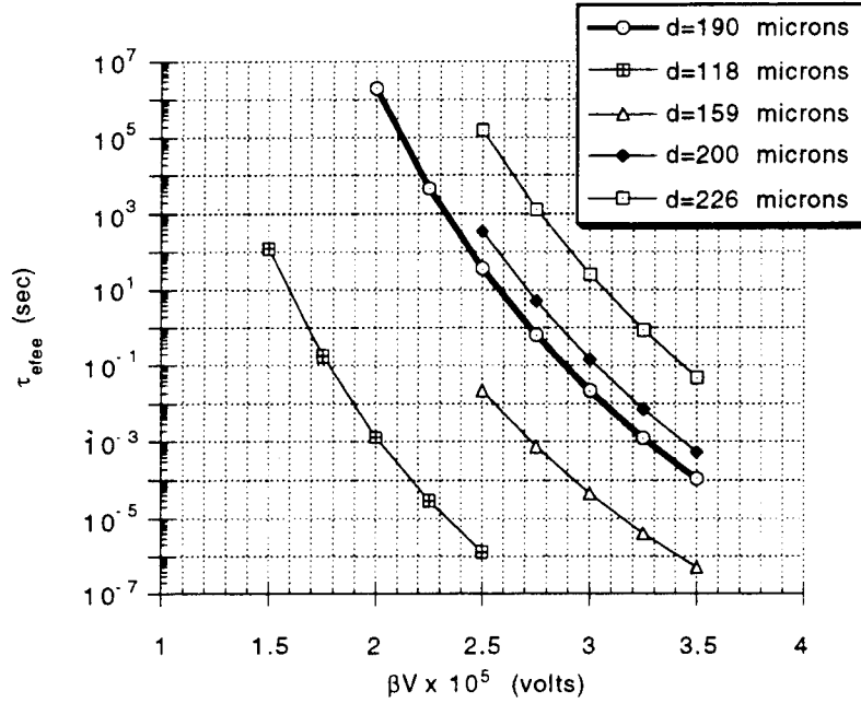
Figure 25: Enhanced field electron emission charging time, \tau_{efee} , versus \beta V for different dielectric thicknesses, d(\mu\text{m})
