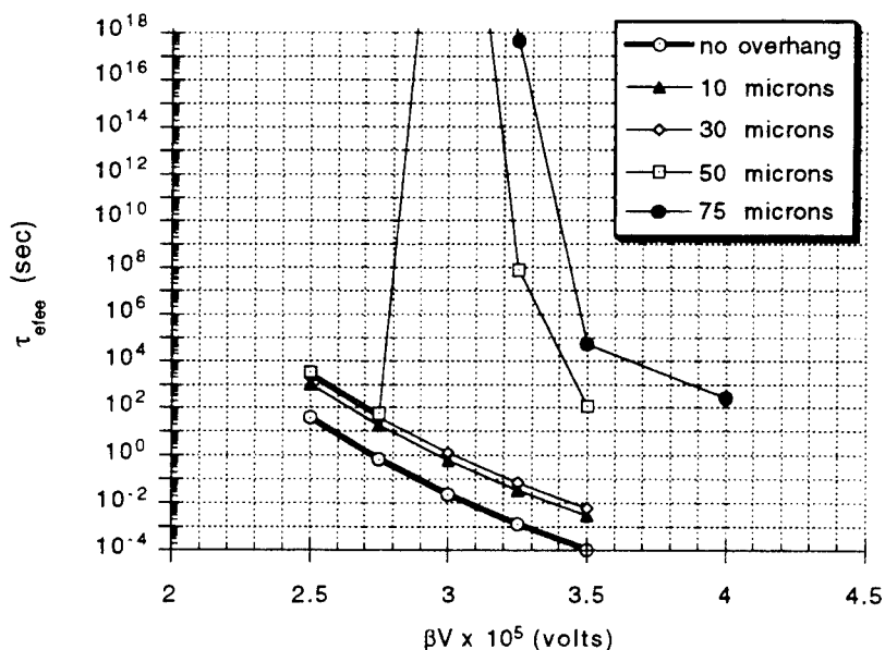
Figure 36: Enhanced field electron emission charging time, \tau_{efee} , versus \beta V for different overhang lengths
