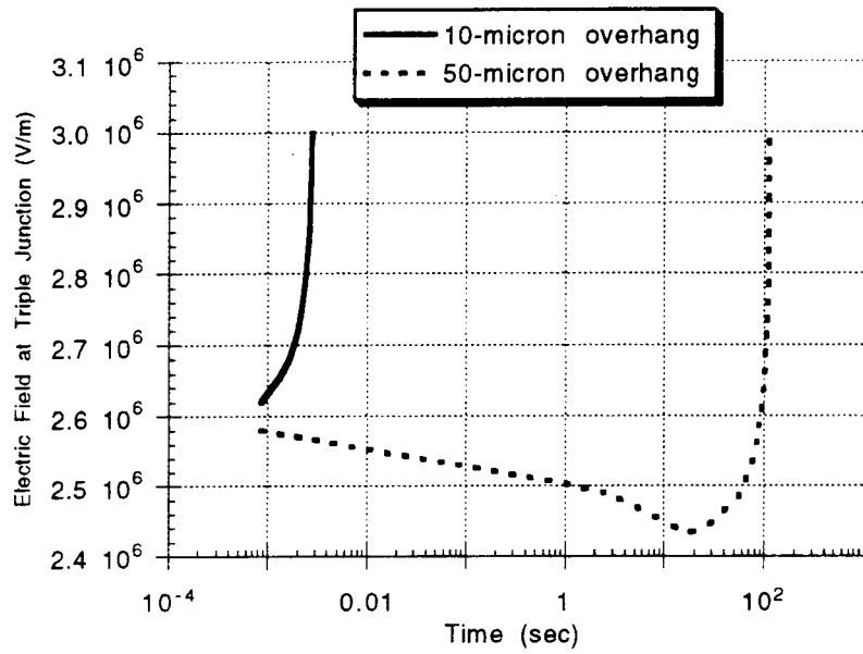
Figure 37: Class comparison of \tau_{efec} versus E_{TJ} for \beta V = 3.5 \times 10^5 \text{V}
