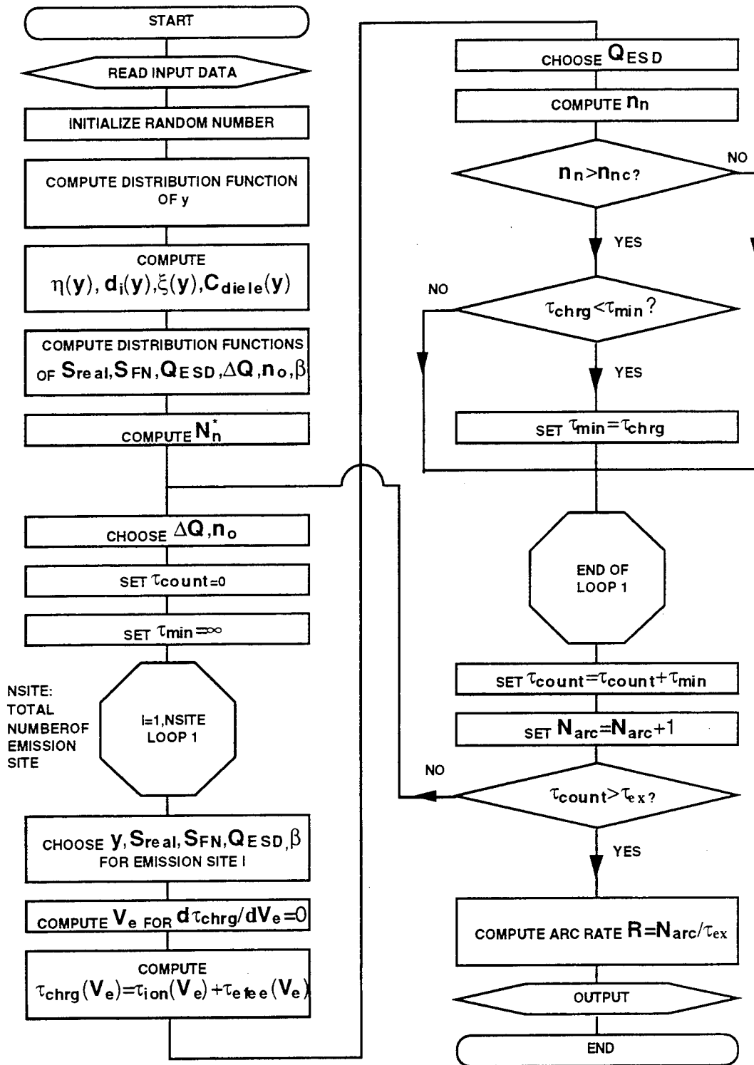
Figure 6: Flow Chart of Semi-Analytic Arc Rate Code
