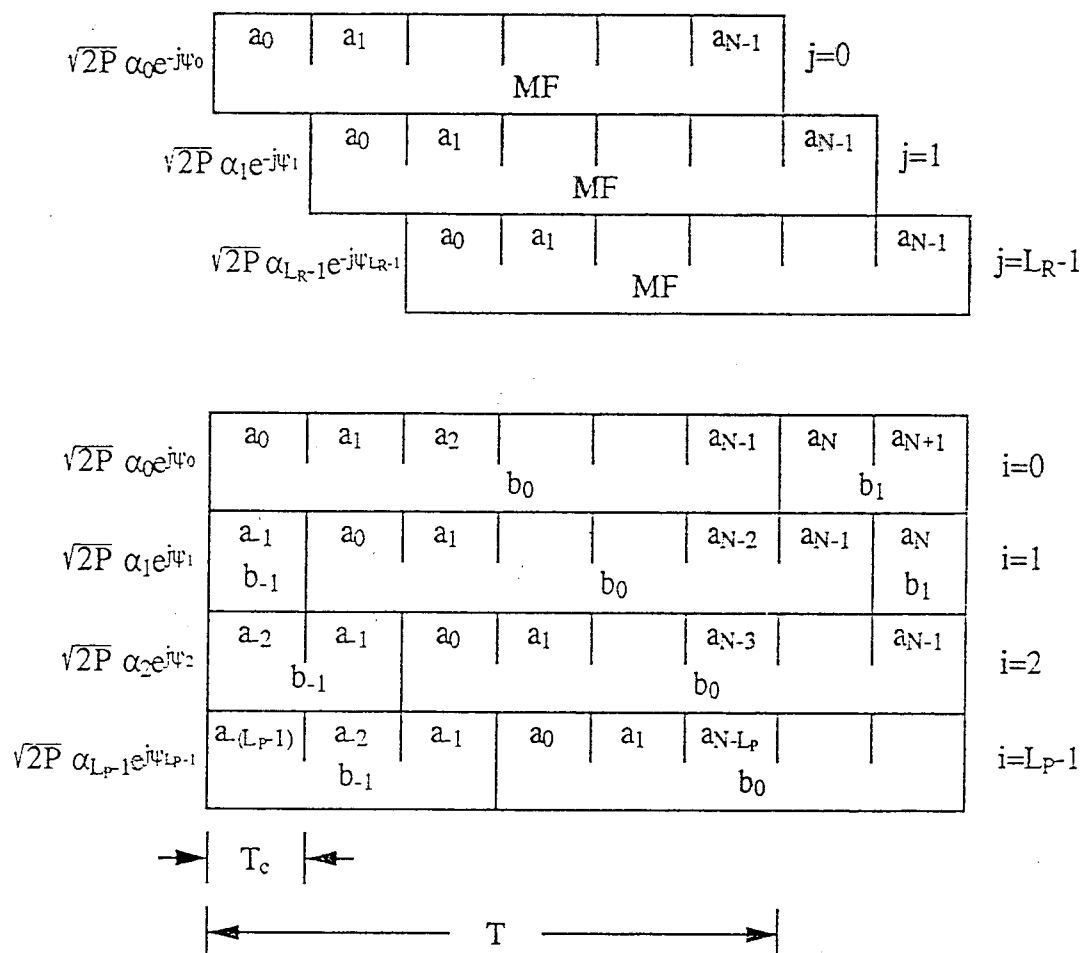
Fig. A1. Pictorial representation of receiver response to reference signal. In this example, the number of paths received is four, and the number of paths combined is three. The response is obtained as follows: For each (i,j) combination, superimpose the two segments by sliding the j -segment down (or by sliding the i -segment up) and integrating the portion that overlaps. Each segment is multiplied by the factor shown to the left of it. Since all the segments are chip synchronized, the integration reduces to a sum of N chips. The response is obtained by summing the contributions from all (i,j) combinations.
