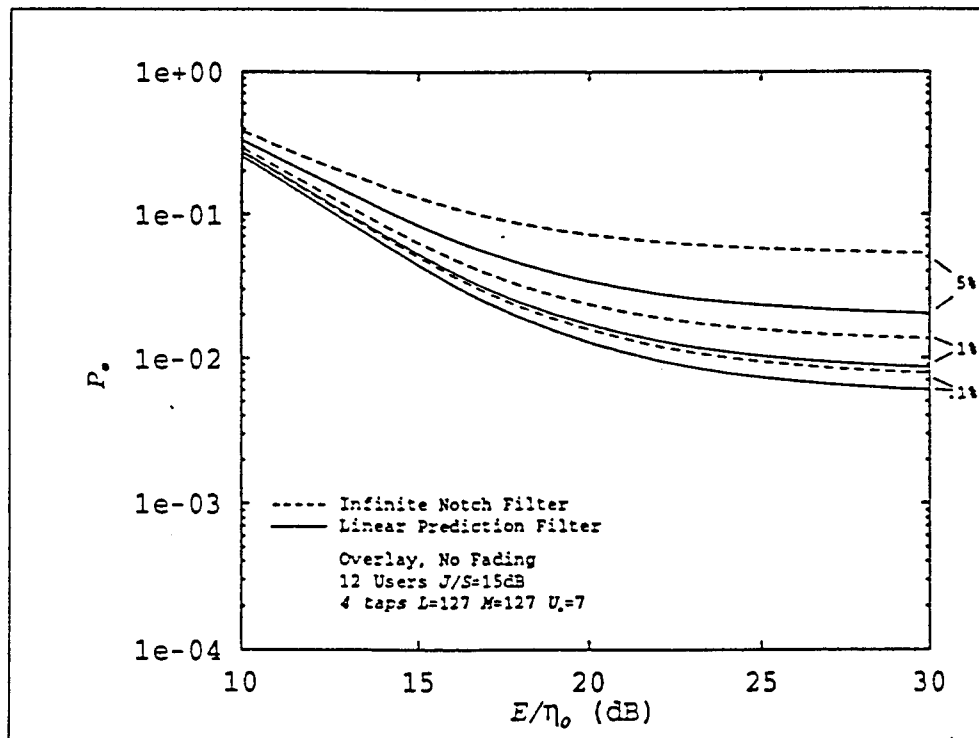
Figure 10 : Analytical Overlay Performance of 4 Tap Infinite Notch System
