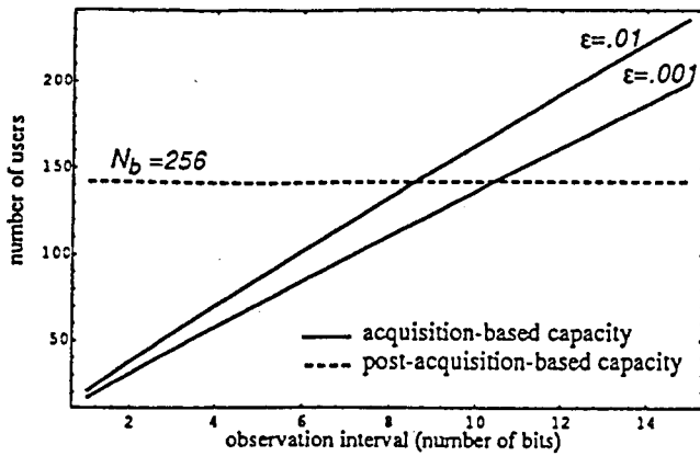
Figure 4: Comparison of the capacity based on acquisition and post acquisition performance criteria. The uncoded bit error rate needs to be less than or equal to 10^{-2} . The probability of false lock needs to be less than or equal to \epsilon . The maximum number of users is plotted versus the observation interval in bits. For comparison, the results are shown for \epsilon = .01, .001 . The number of chips per bit is 256.
