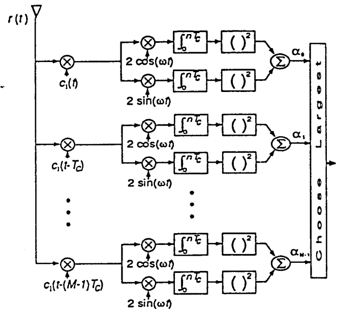
Figure 1: Coarse Acquisition Circuitry: A bank of I-Q noncoherent detectors is used to simultaneously test the spreading sequence phases within the uncertainty region.
