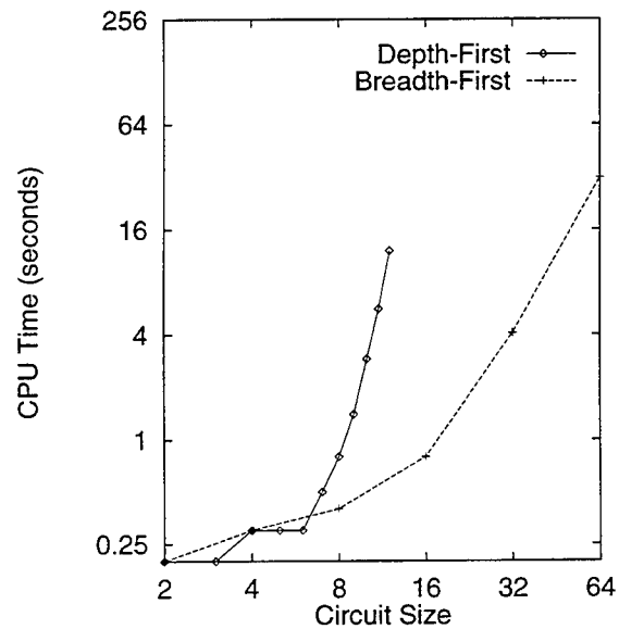
Figure 6.15: LIF Equivalence for Counters: Depth-first vs. Breadth-first
