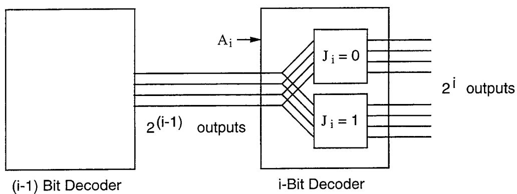
Figure 4.21: Parametric Description of a Decoder
