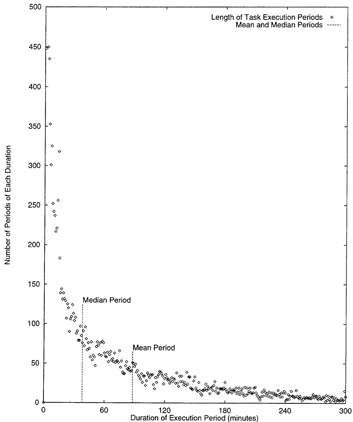
Figure 6.2: This graph shows the distribution of the length of time a task was able to execute before terminating or being interrupted. This data covers all machines that have been used to process Wax tasks. The graph covers about 15,000 execution periods. The point for the two minute execution periods, which is off the top of the chart, is at 791.
