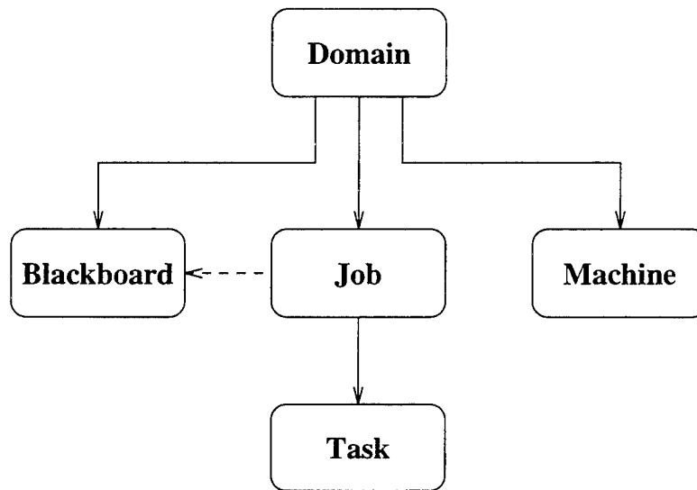
Figure 4.3: The ACL hierarchy supported by Wax . Starting from the top, the solid arrows indicate the sequence of ACLs that must be checked in order to access each type of object. The dashed arrow between a job and a blackboard is there because while a blackboard can be accessed independently from the job(s) that use it, access to a job is necessary in order to examine the list of blackboards it uses, which is generally a pre-cursor to accessing a blackboard.
