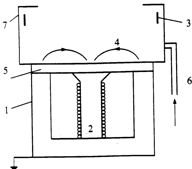
Figure 3. 1—cathode of the magnetron, 2—cylindrical electromagnet, 3—anode, 4—magnetic flux lines, 5—sputtered target, 6—gas duct
