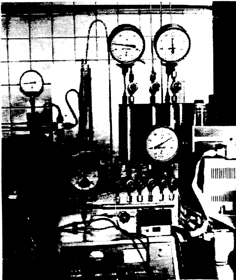
Photograph 4. An installation for plasma assisted CVD
