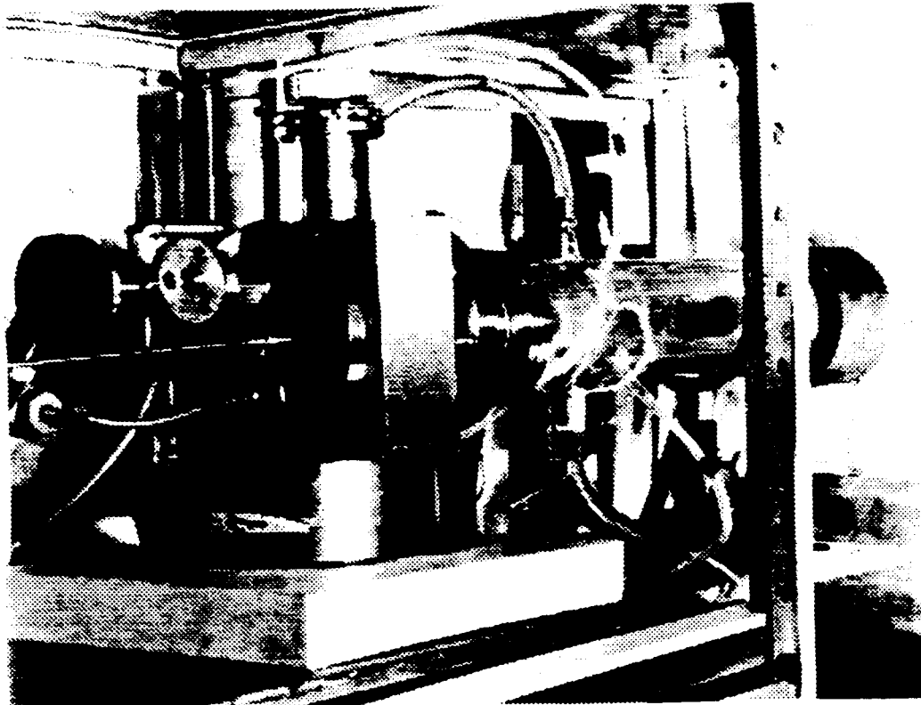
Photograph 1. An installation for growing epitaxial SiC layers by CVD
