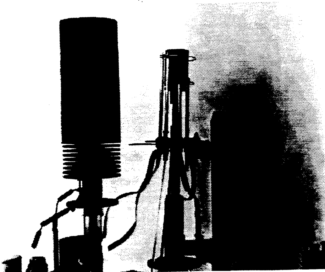
Photograph 2. An installation for growing epitaxial SiC layers by sublimation with electron heated cell
