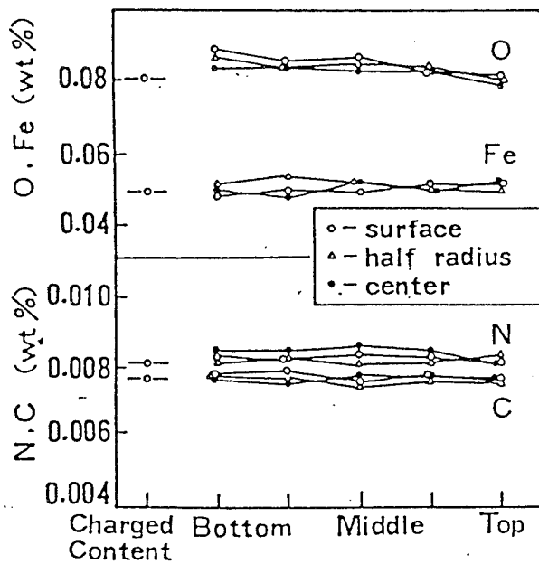
Distribution of chemical compositions in a pure titanium ingot. Titanium scrap ratio; 50%
