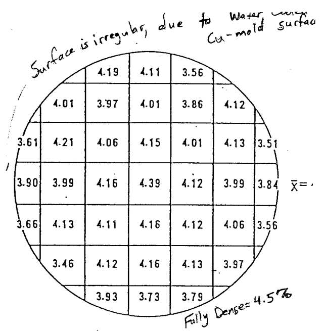
Density distribution of a PPC titanium ingot. Melting power; 380 kW, Melting speed; 4 kg/min., Sponge-Ti ratio; 50%
