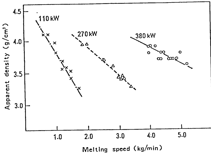
Relation between the melting speed and the ingot density.
