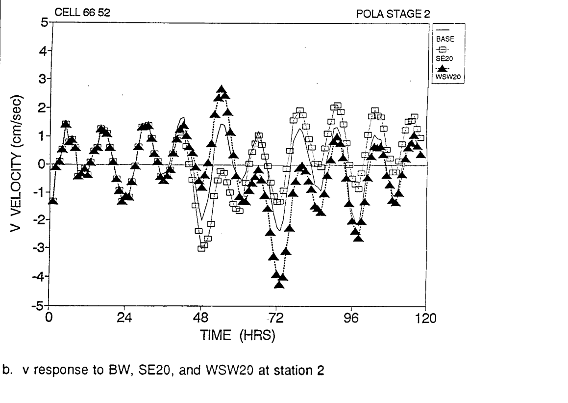
Figure D14. Time series of POLA 2 current velocity
