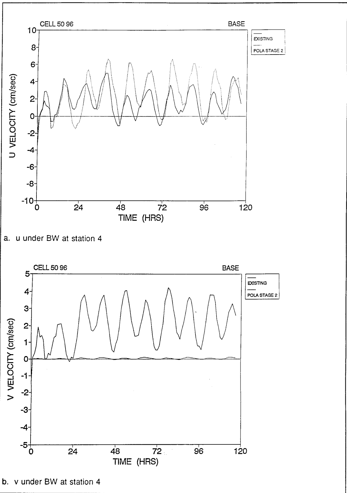
Figure D12. Time series of POLA 2 current velocity
