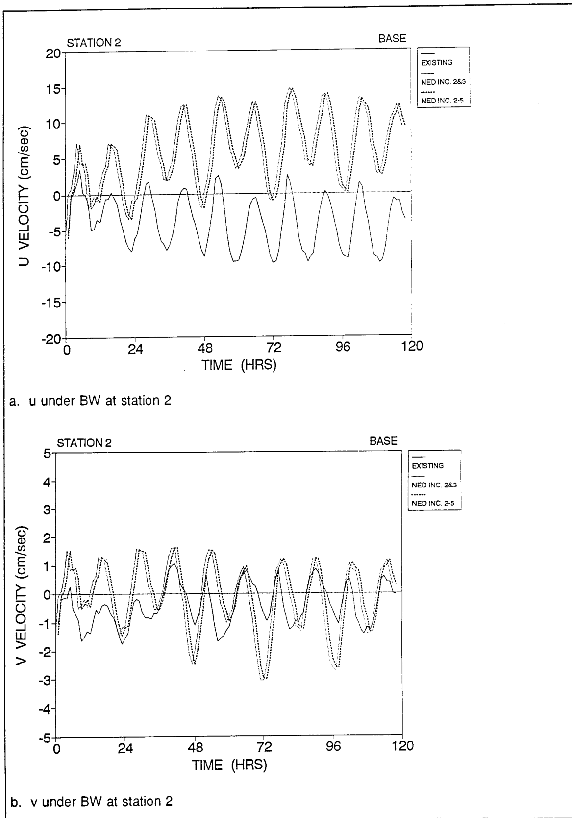
Figure D26. Time series of NED2&3 and NED2-5 current velocity
