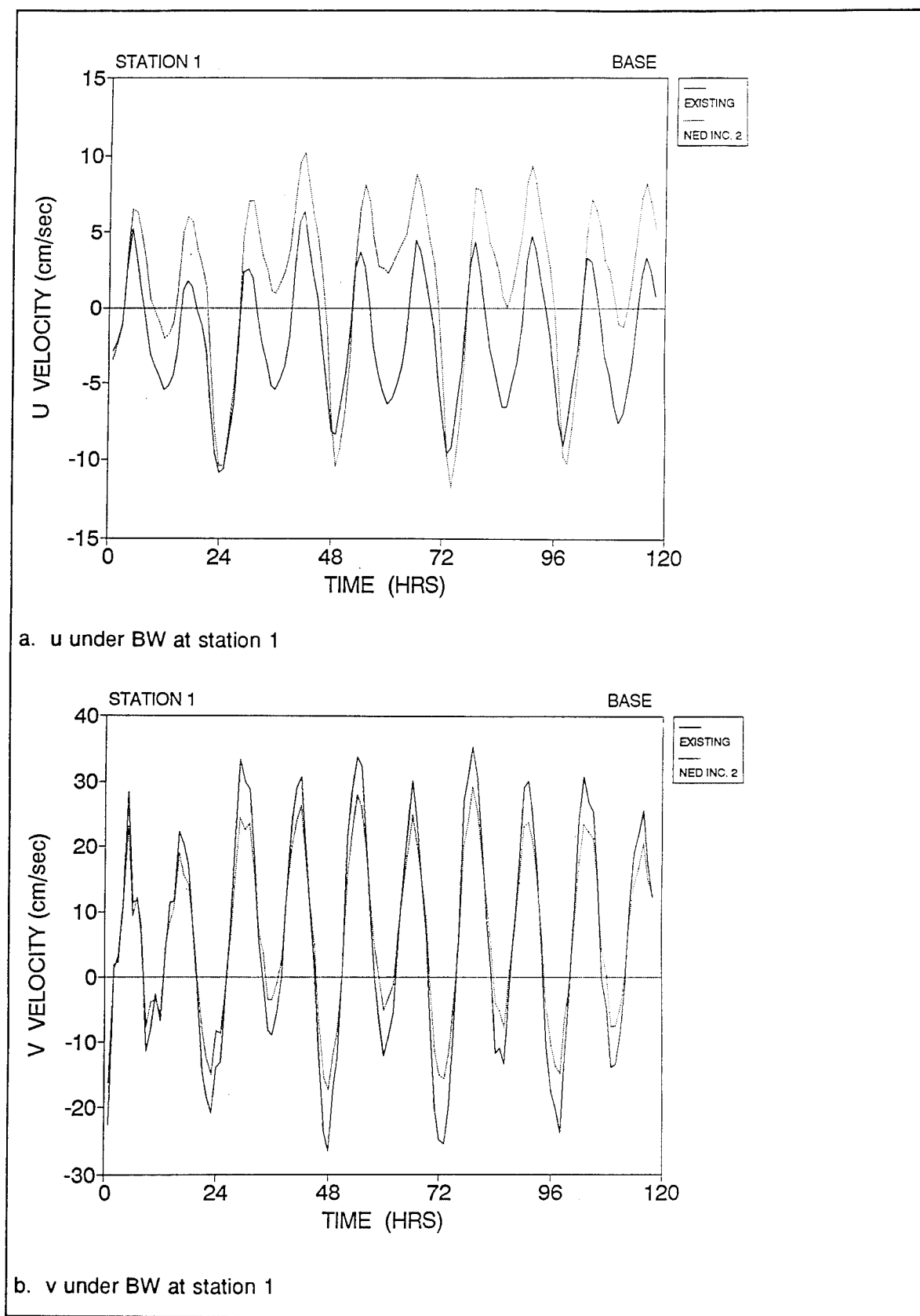
Figure D17. Time series of NED2 current velocity
