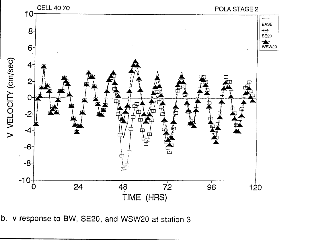
Figure D15. Time series of POLA 2 current velocity
